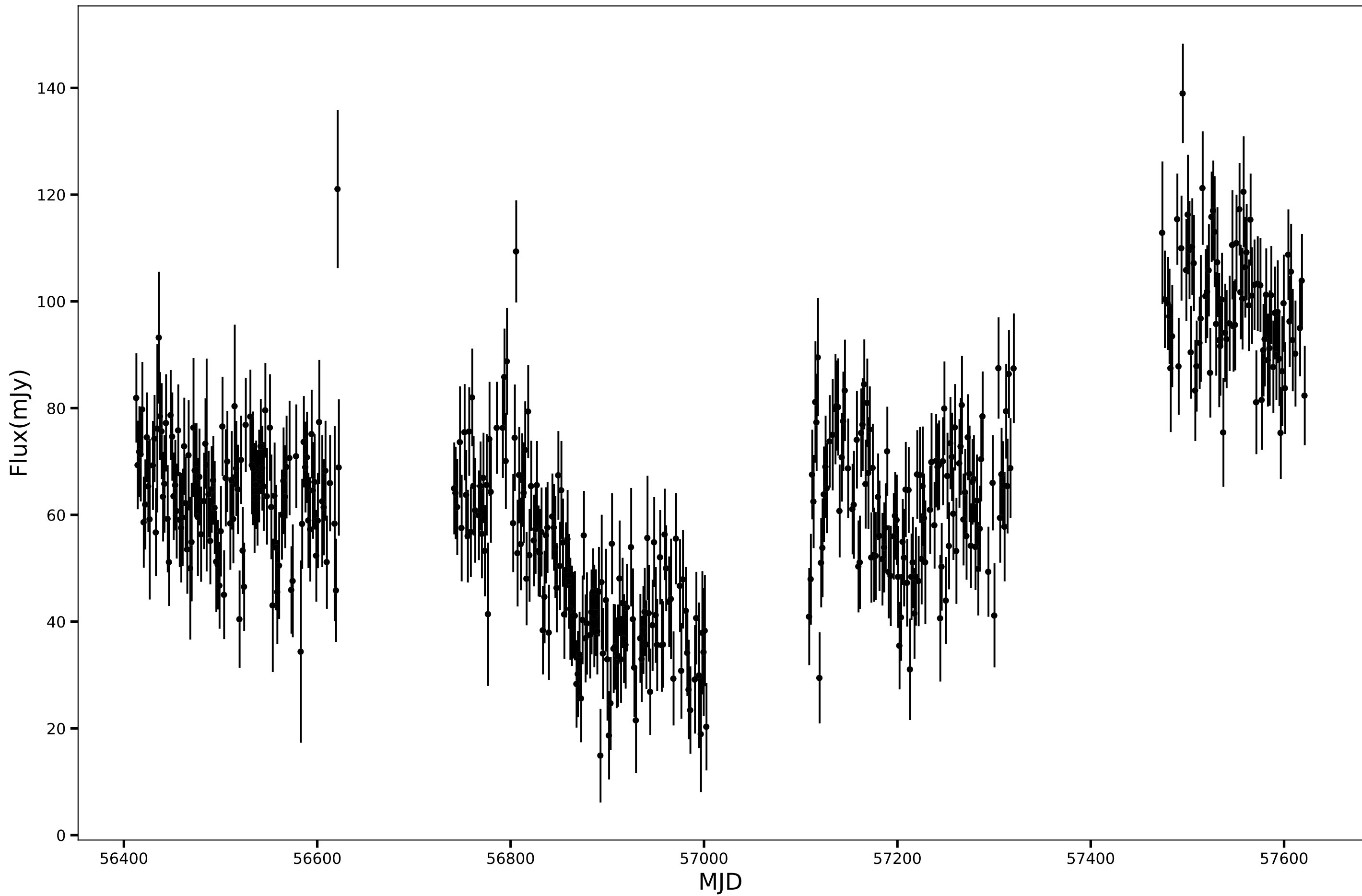
SPT-SJ223422-5405.9, RA=338.5945d, DEC=-54.0998d, mean_flux=65.22 (mJy), 150GHz
