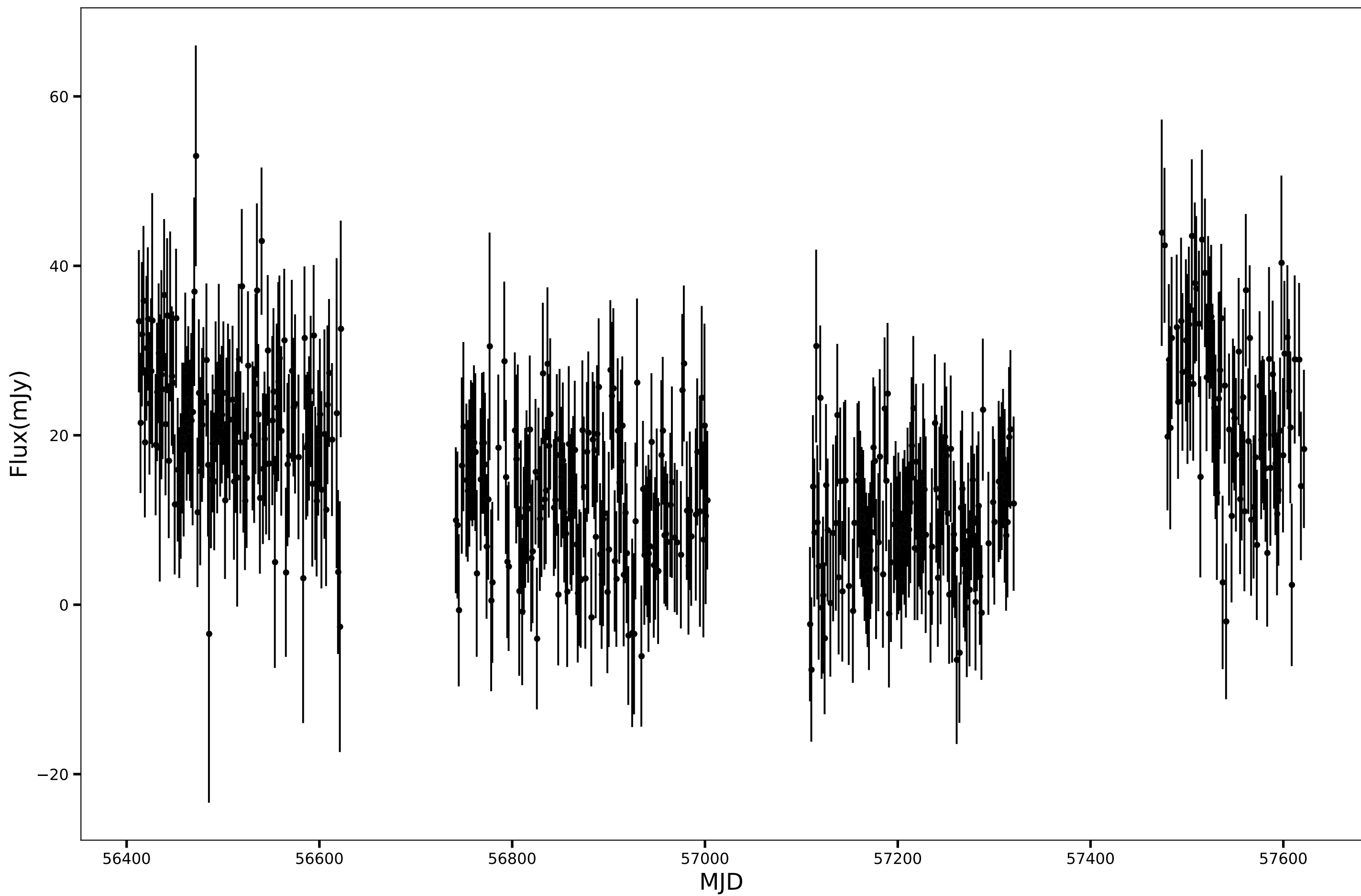
SPT-SJ223044-6329.4, RA=337.6842d, DEC=-63.4901d, mean_flux=16.12 (mJy), 150GHz
