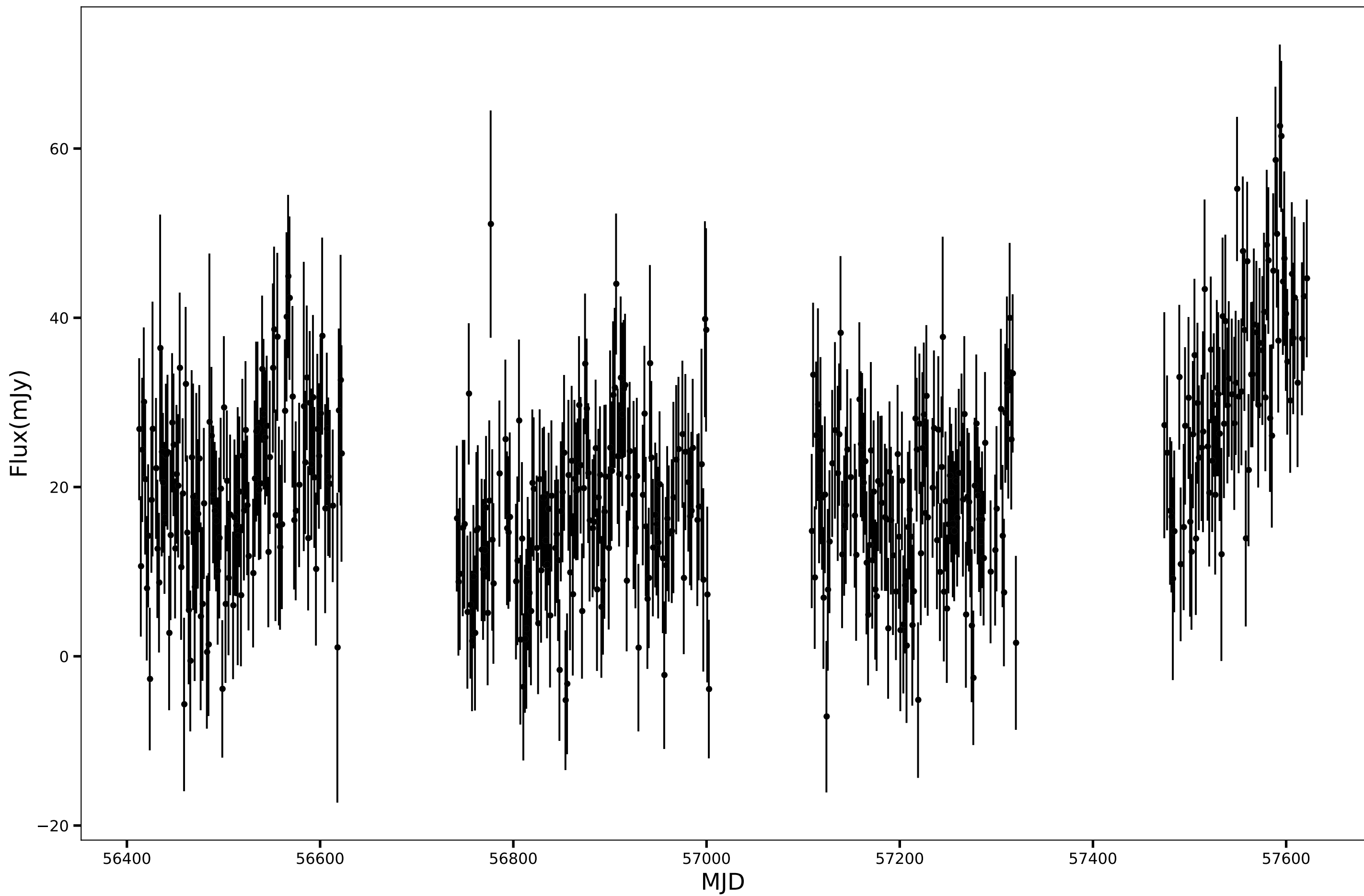
SPT-SJ223042-5415.2, RA=337.6771d, DEC=-54.2549d, mean_flux=20.39 (mJy), 150GHz
