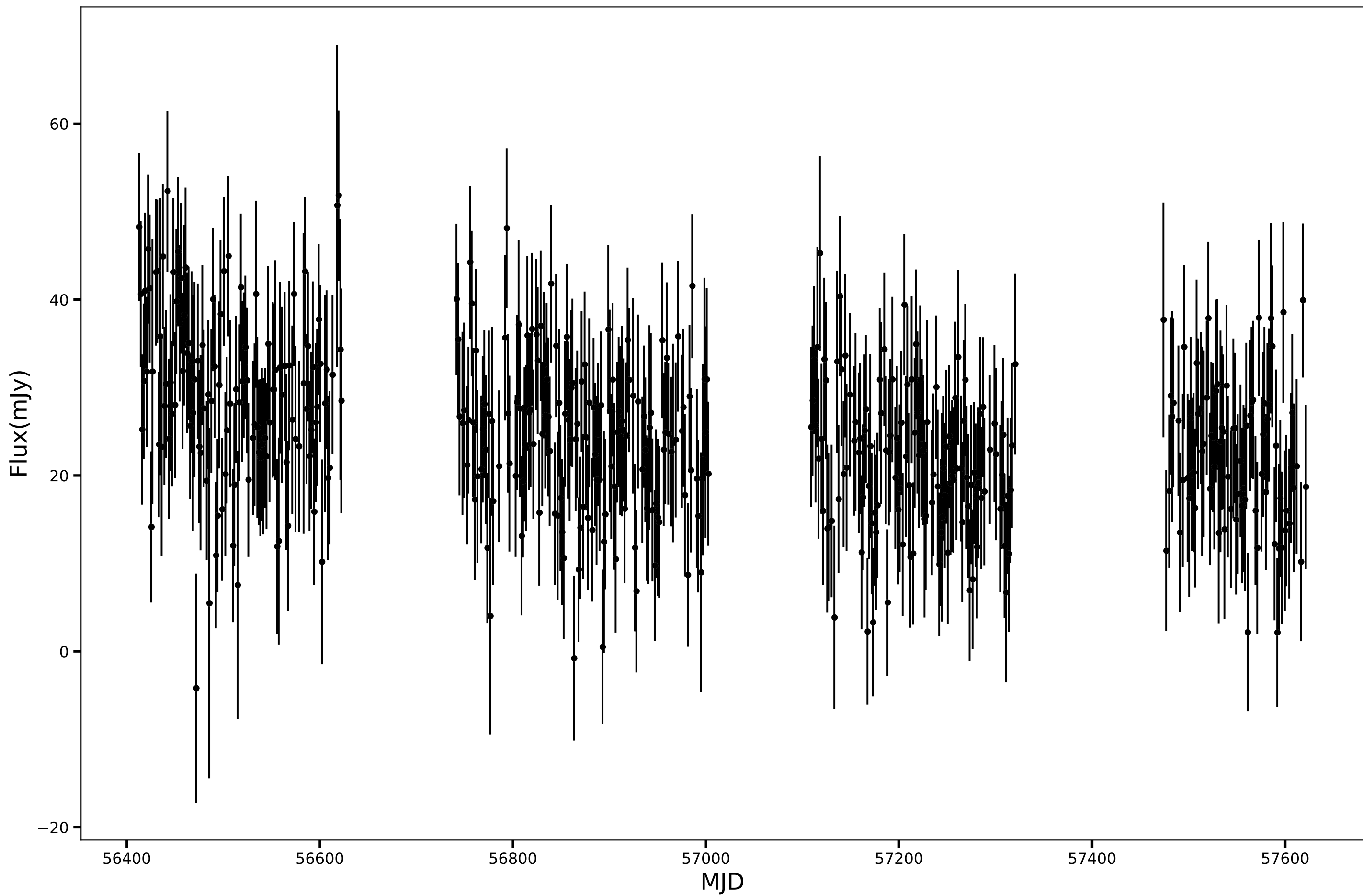
SPT-SJ223011-6310.7, RA=337.5466d, DEC=-63.1786d, mean_flux=24.60 (mJy), 150GHz
