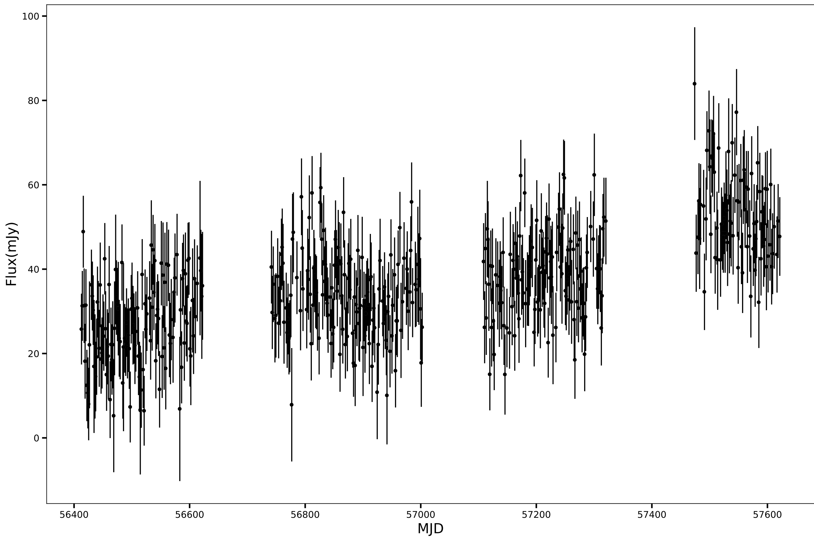
SPT-SJ222707-5219.9, RA=336.7831d, DEC=-52.3329d, mean_flux=36.49 (mJy), 150GHz
