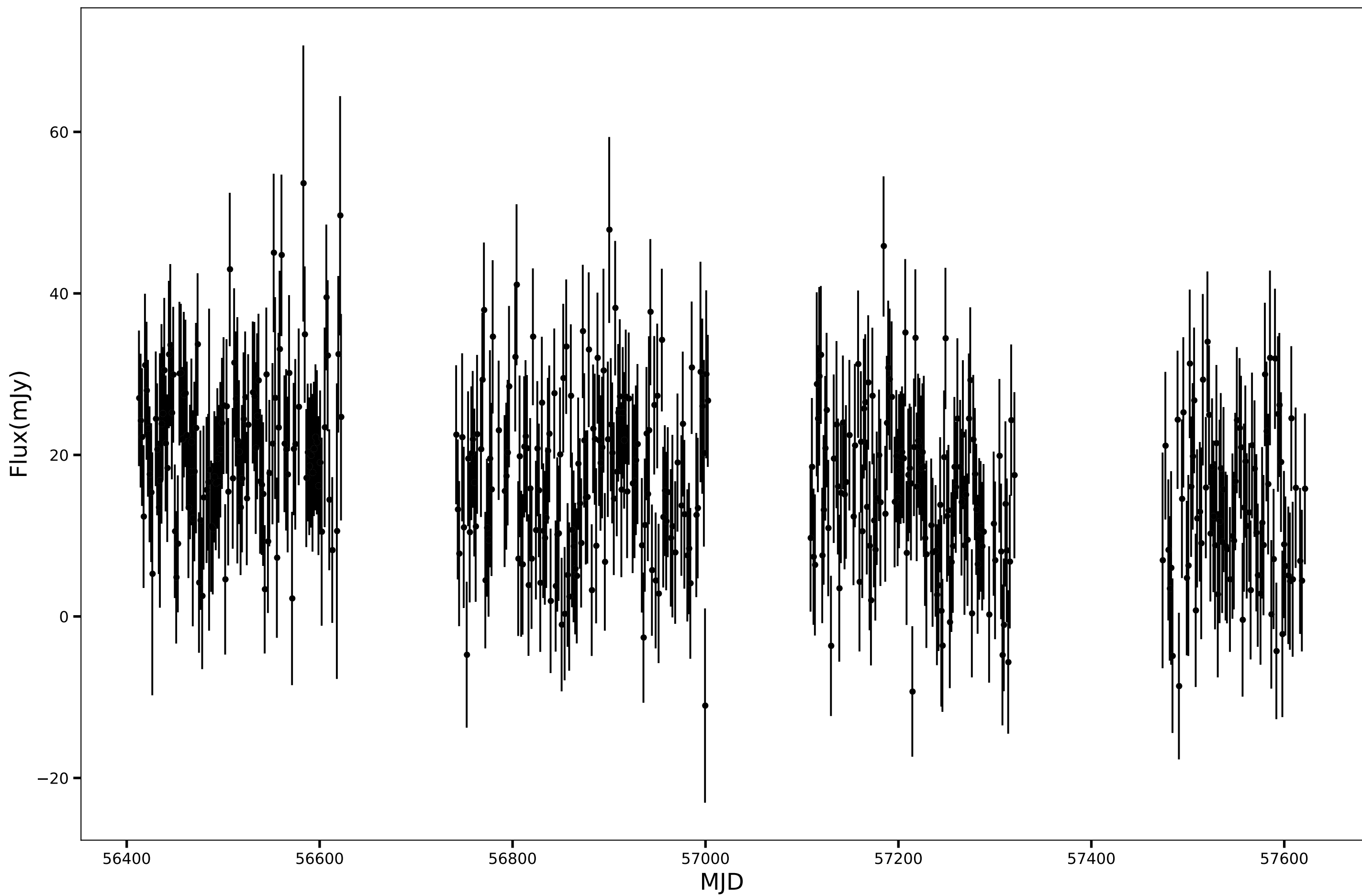
SPT-SJ221818-5038.6, RA=334.5765d, DEC=-50.6445d, mean_flux=17.22 (mJy), 150GHz
