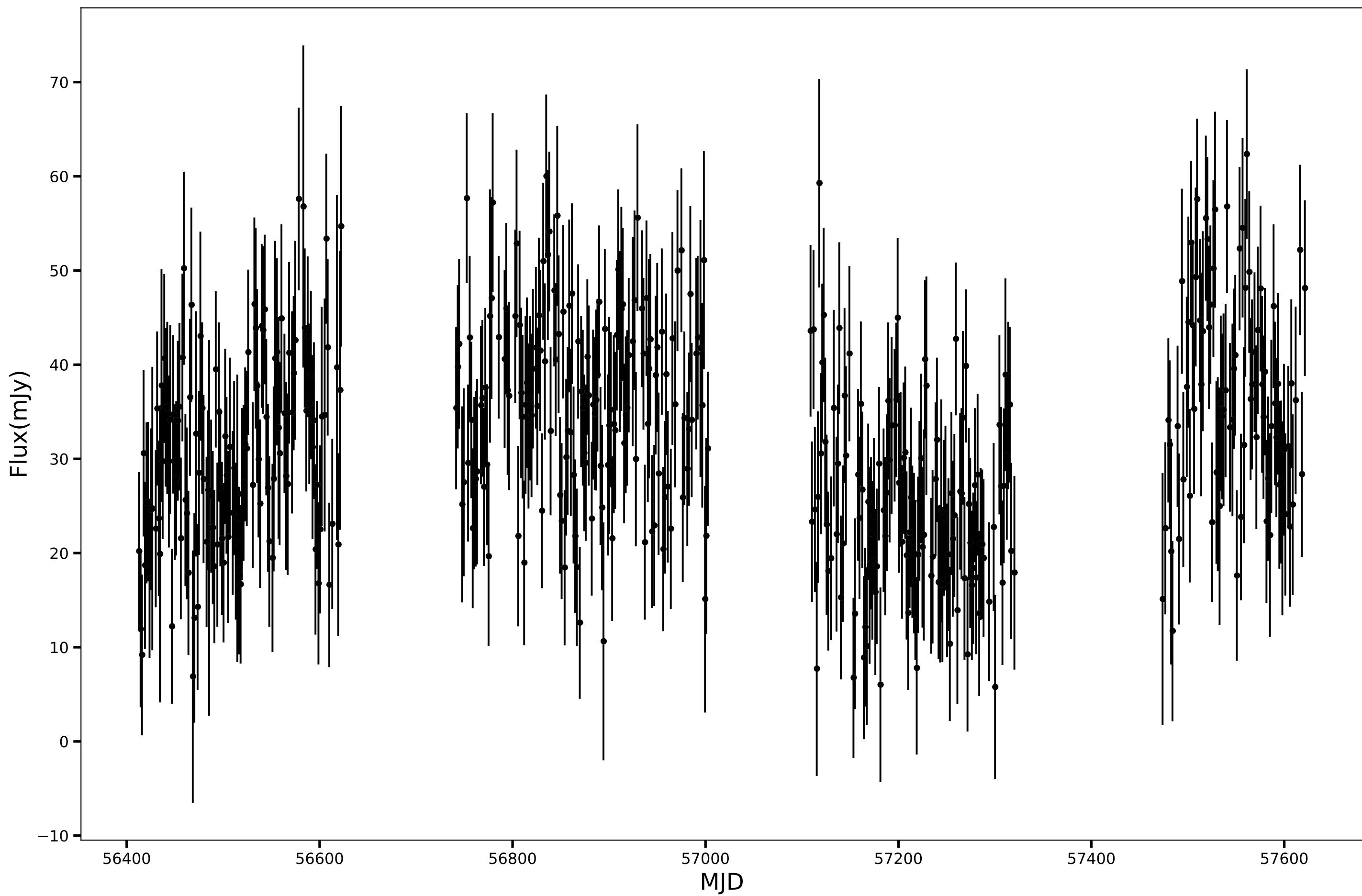
SPT-SJ221642-5637.5, RA=334.1768d, DEC=-56.6259d, mean_flux=31.89 (mJy), 150GHz
