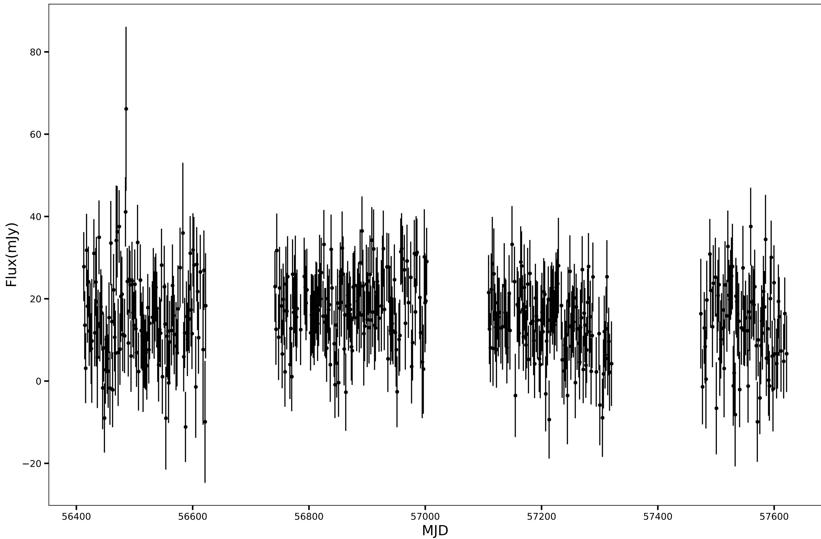
SPT-SJ221623-5238.0, RA=334.0998d, DEC=-52.6334d, mean_flux=15.49 (mJy), 150GHz
