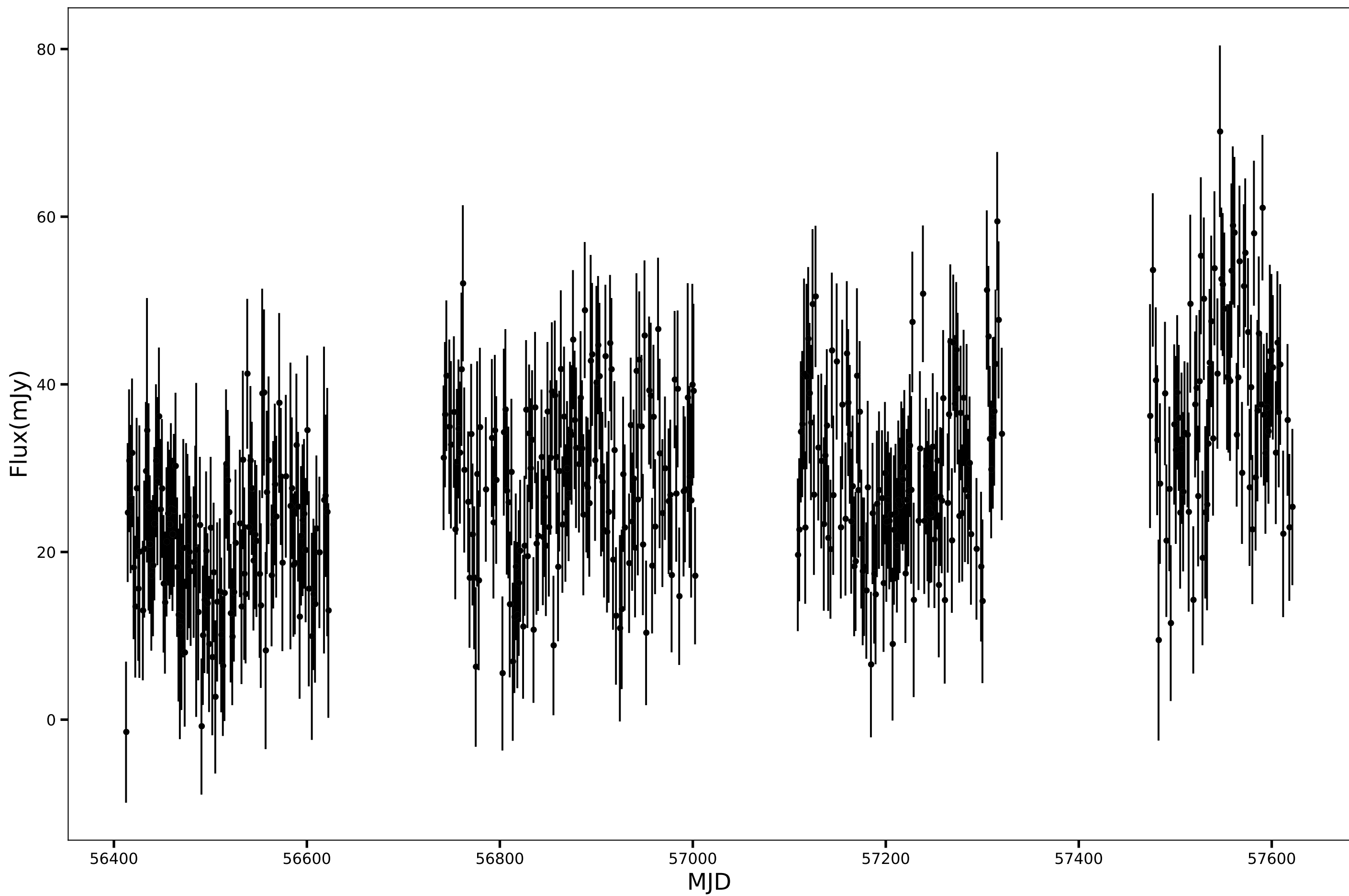
SPT-SJ221032-5508.6, RA=332.6343d, DEC=-55.1437d, mean_flux=28.55 (mJy), 150GHz
