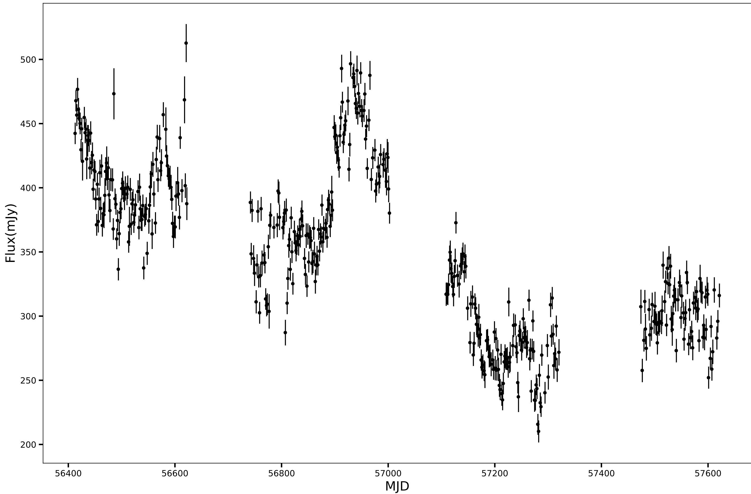
SPT-SJ220743-5346.5, RA=331.9309d, DEC=-53.7760d, mean_flux=350.64 (mJy), 150GHz
