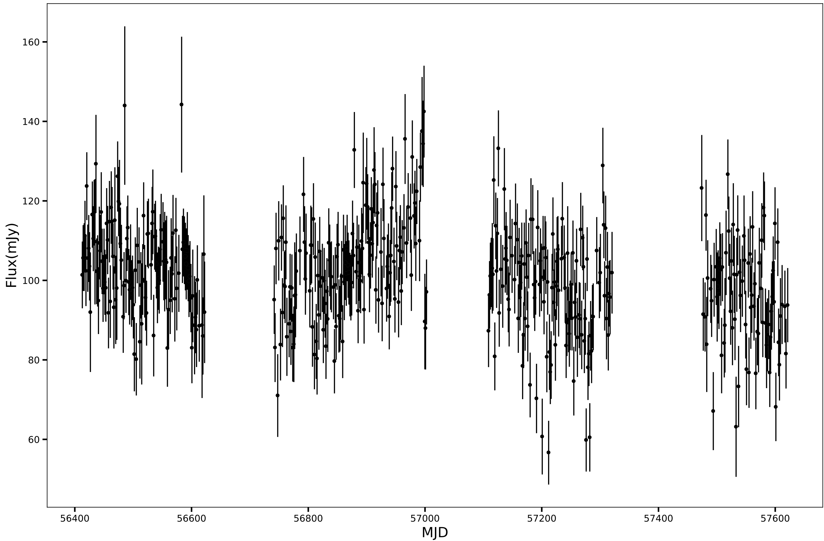
SPT-SJ220359-6130.3, RA=330.9998d, DEC=-61.5067d, mean_flux=100.84 (mJy), 150GHz
