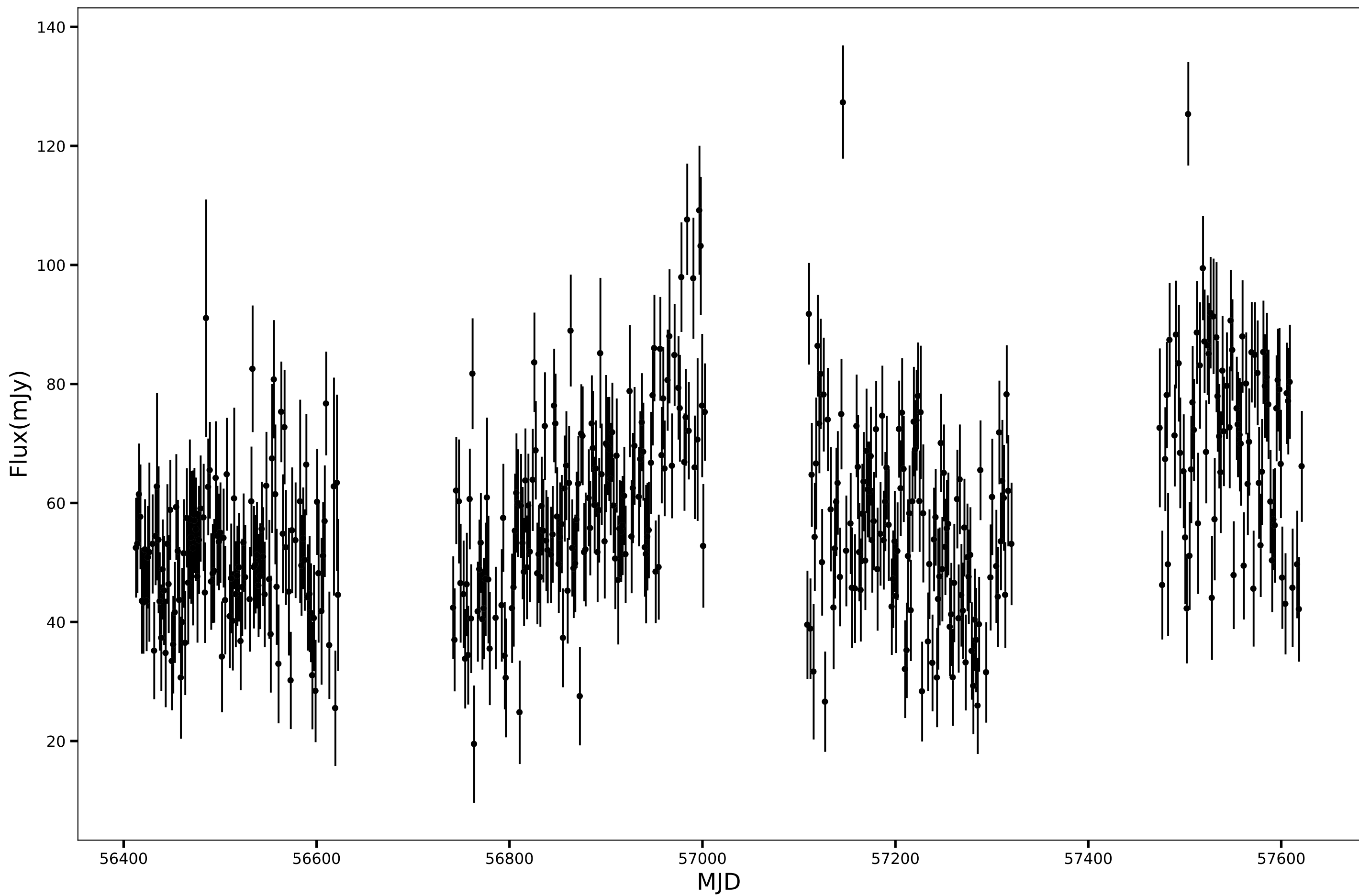
SPT-SJ220301-4937.0, RA=330.7559d, DEC=-49.6173d, mean_flux=58.29 (mJy), 150GHz
