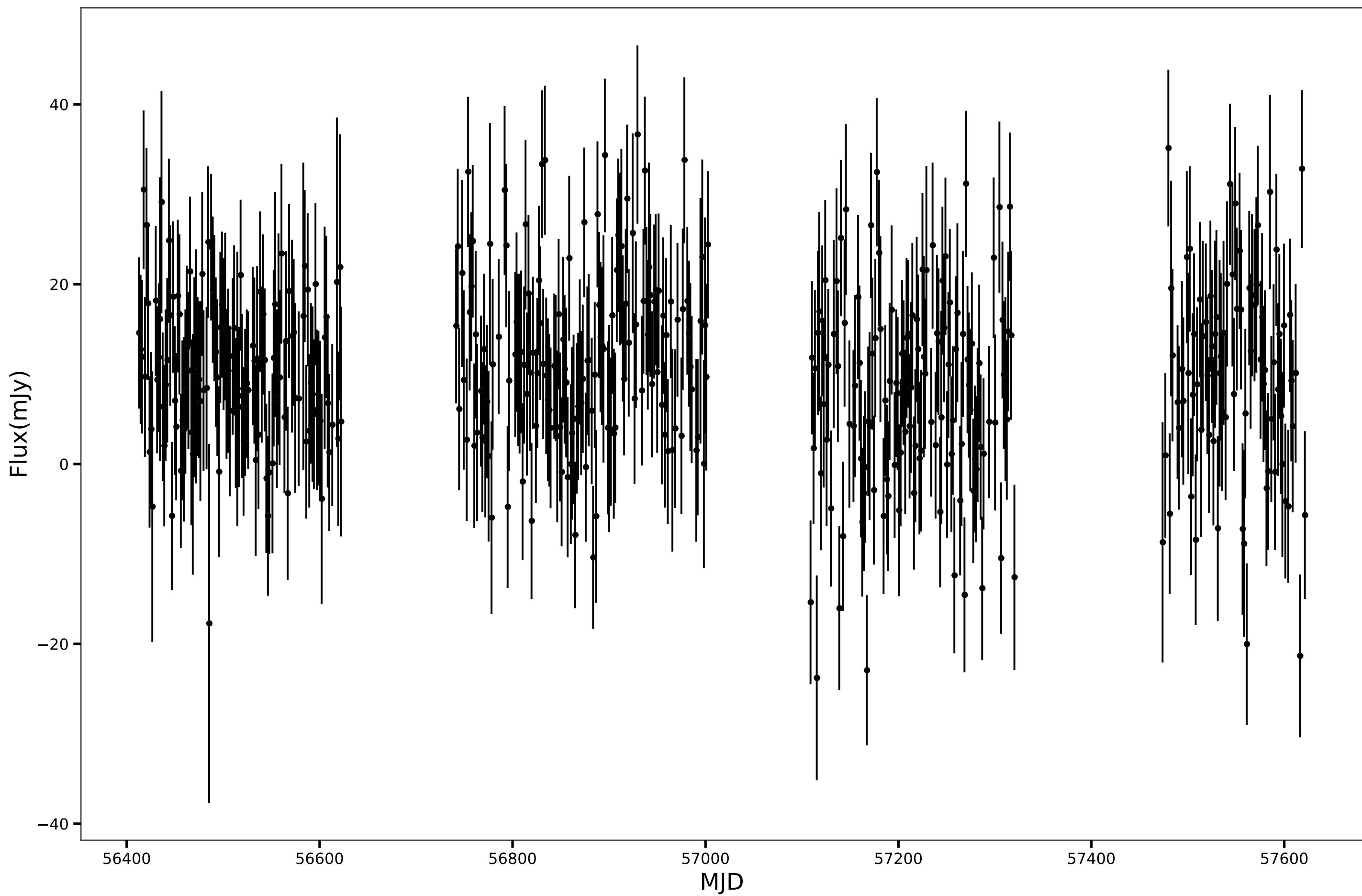
SPT-SJ220145-6457.6, RA=330.4402d, DEC=-64.9604d, mean_flux=10.17 (mJy), 150GHz
