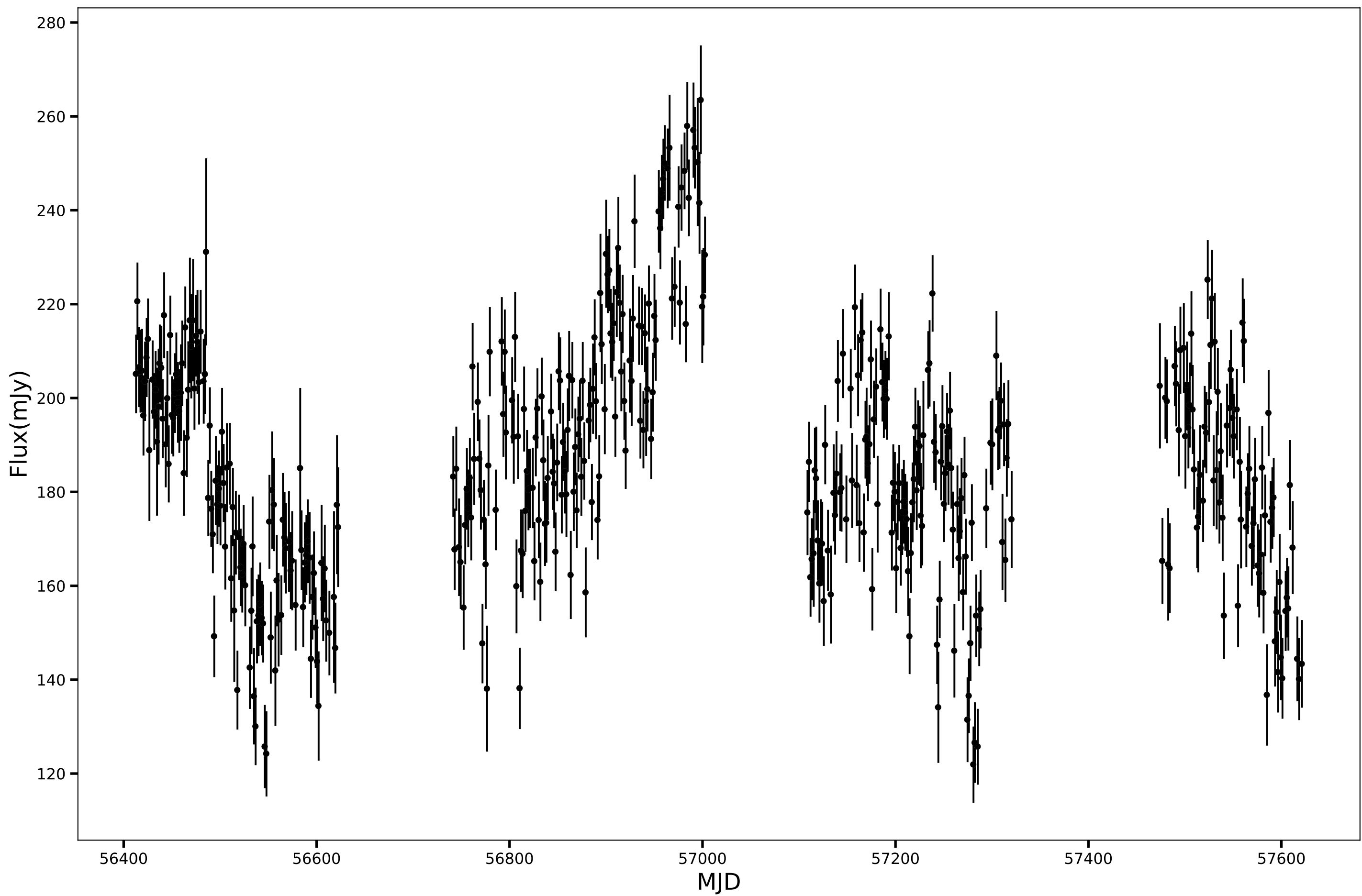
SPT-SJ220055-5520.1, RA=330.2306d, DEC=-55.3356d, mean_flux=185.76 (mJy), 150GHz
