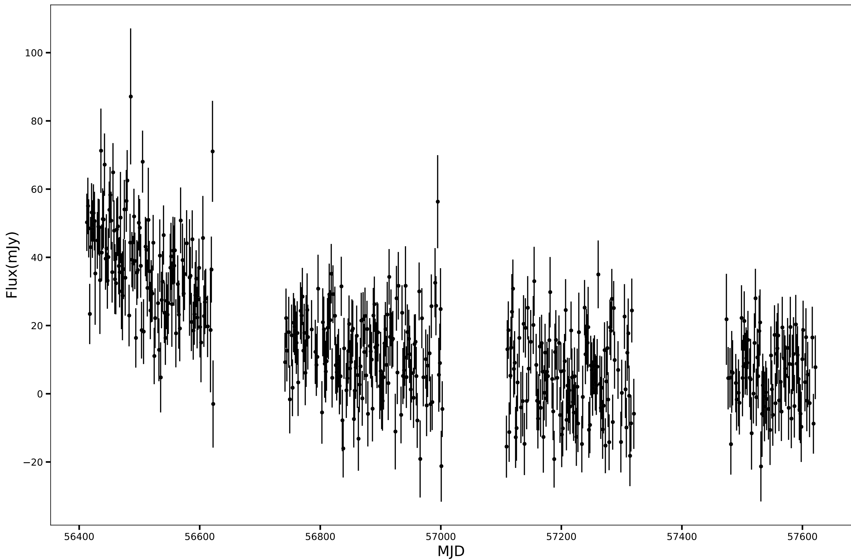
SPT-SJ215648-6331.0, RA=329.2009d, DEC=-63.5179d, mean_flux=15.69 (mJy), 150GHz
