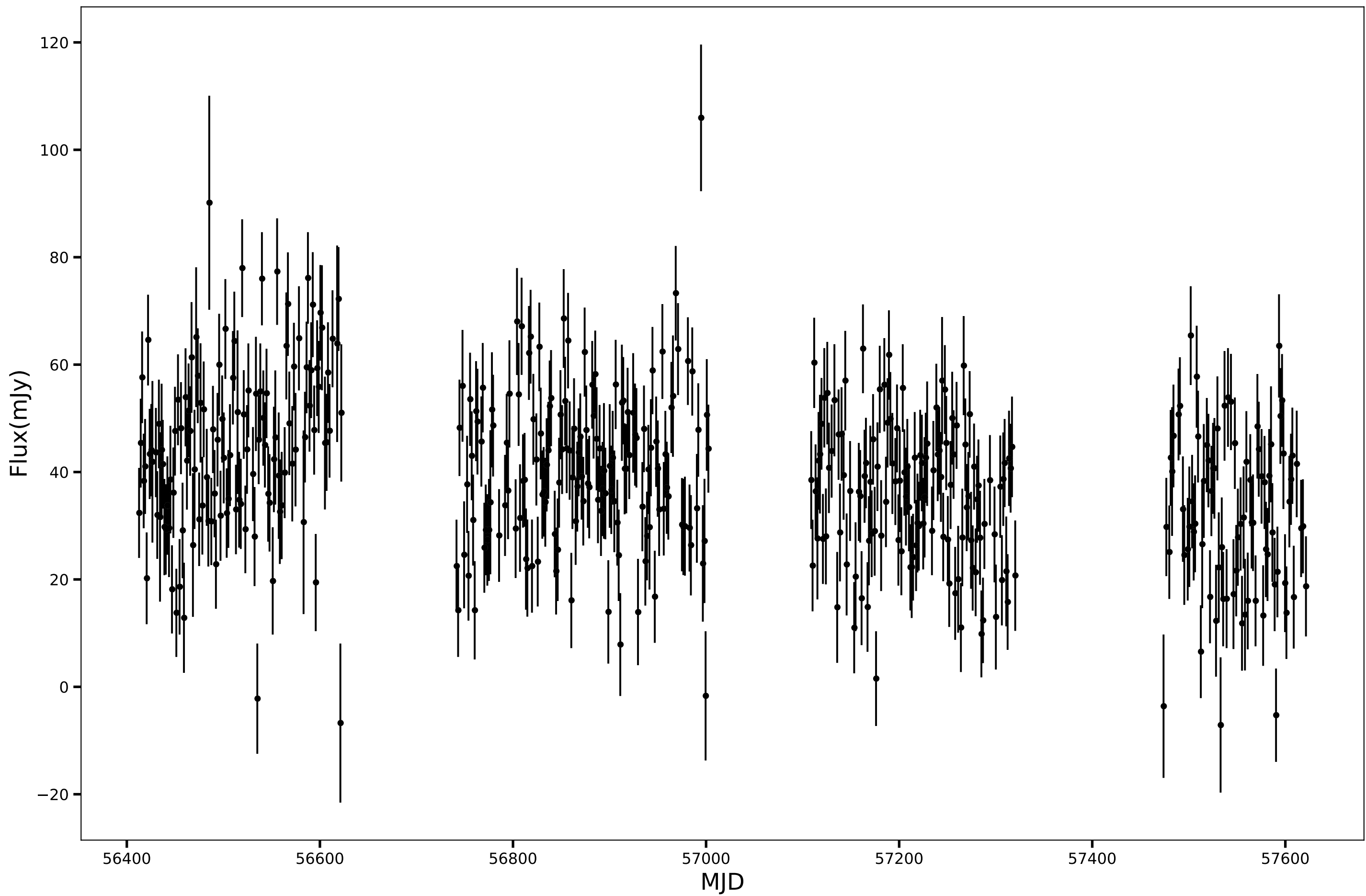
SPT-SJ215543-5400.2, RA=328.9295d, DEC=-54.0034d, mean_flux=39.16 (mJy), 150GHz
