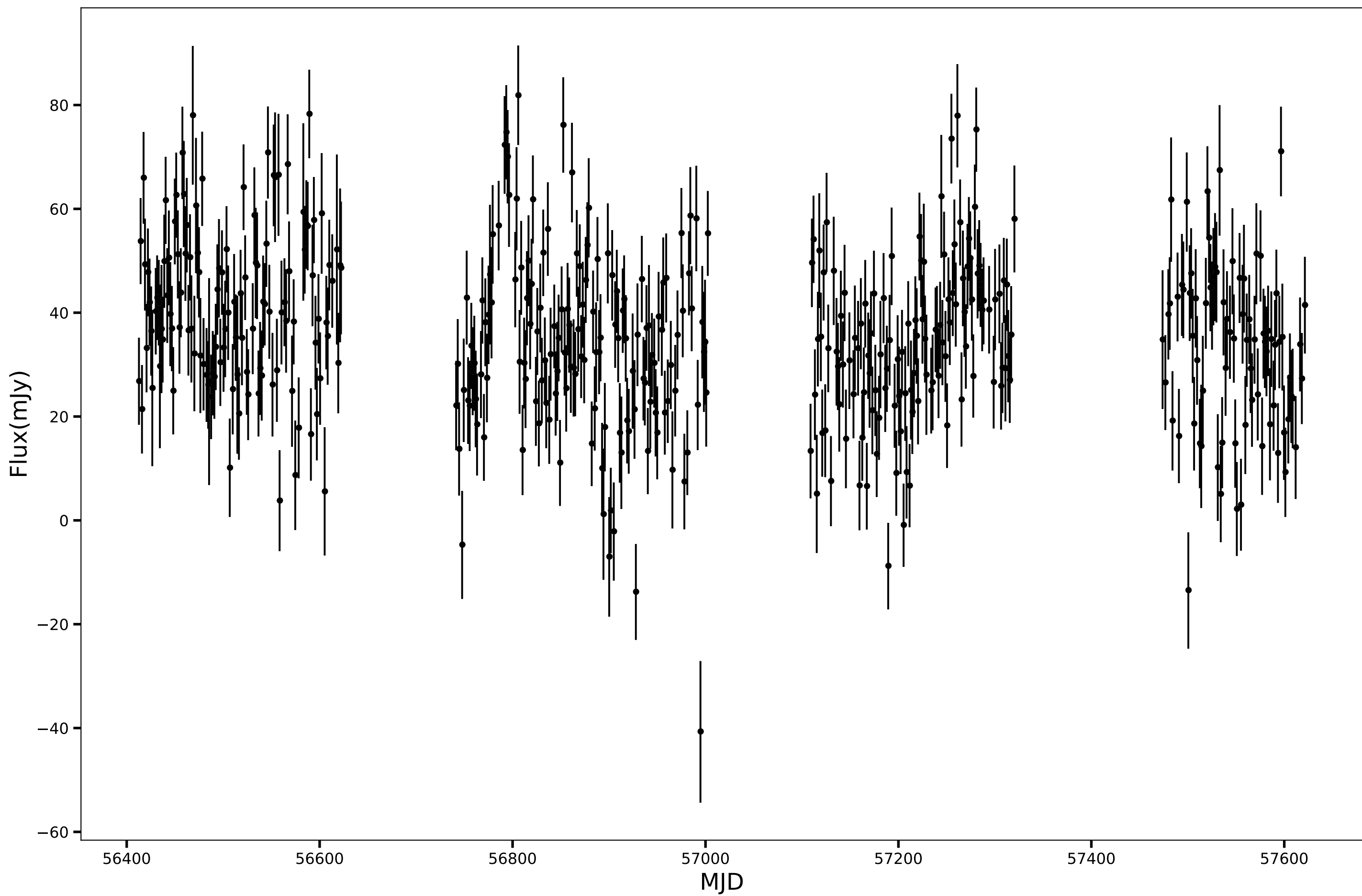
SPT-SJ215445-5725.6, RA=328.6913d, DEC=-57.4277d, mean_flux=35.76 (mJy), 150GHz
