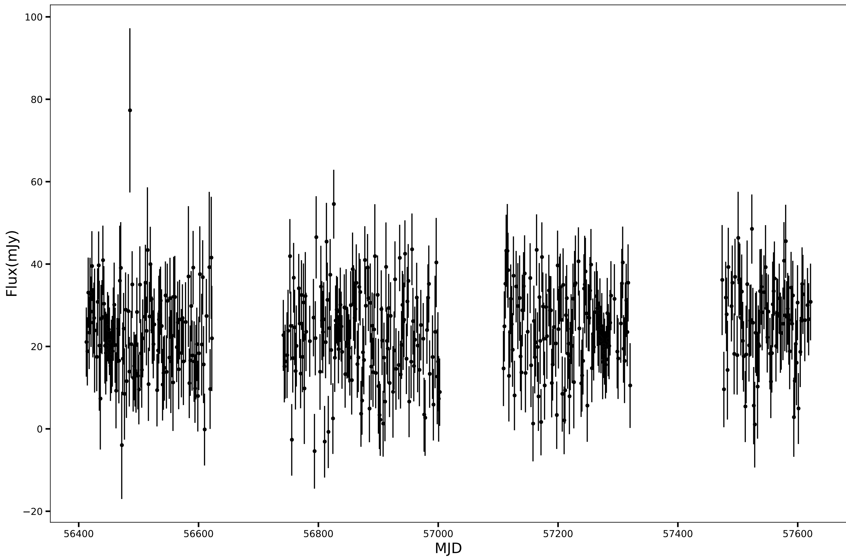
SPT-SJ015853-6334.8, RA=29.7244d, DEC=-63.5801d, mean_flux=23.71 (mJy), 150GHz
