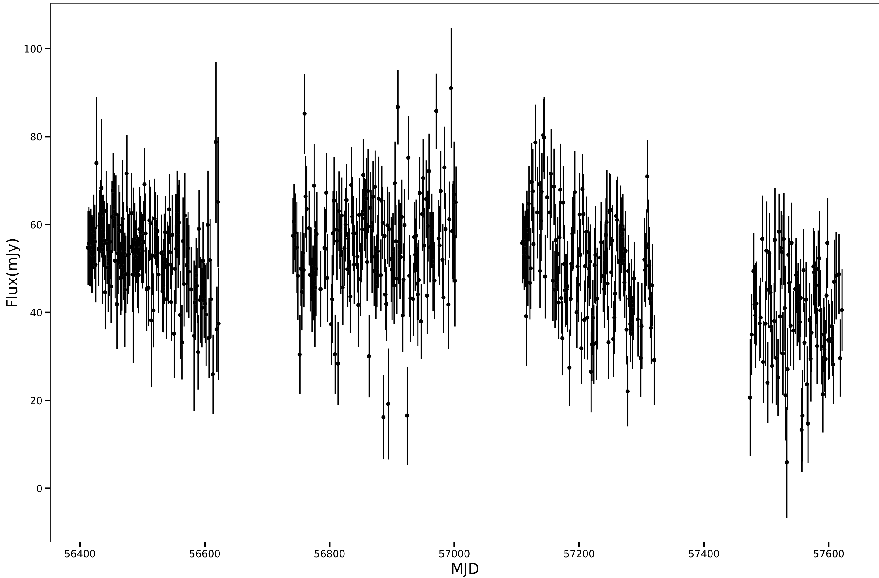
SPT-SJ015836-6411.4, RA=29.6500d, DEC=-64.1914d, mean_flux=50.44 (mJy), 150GHz
