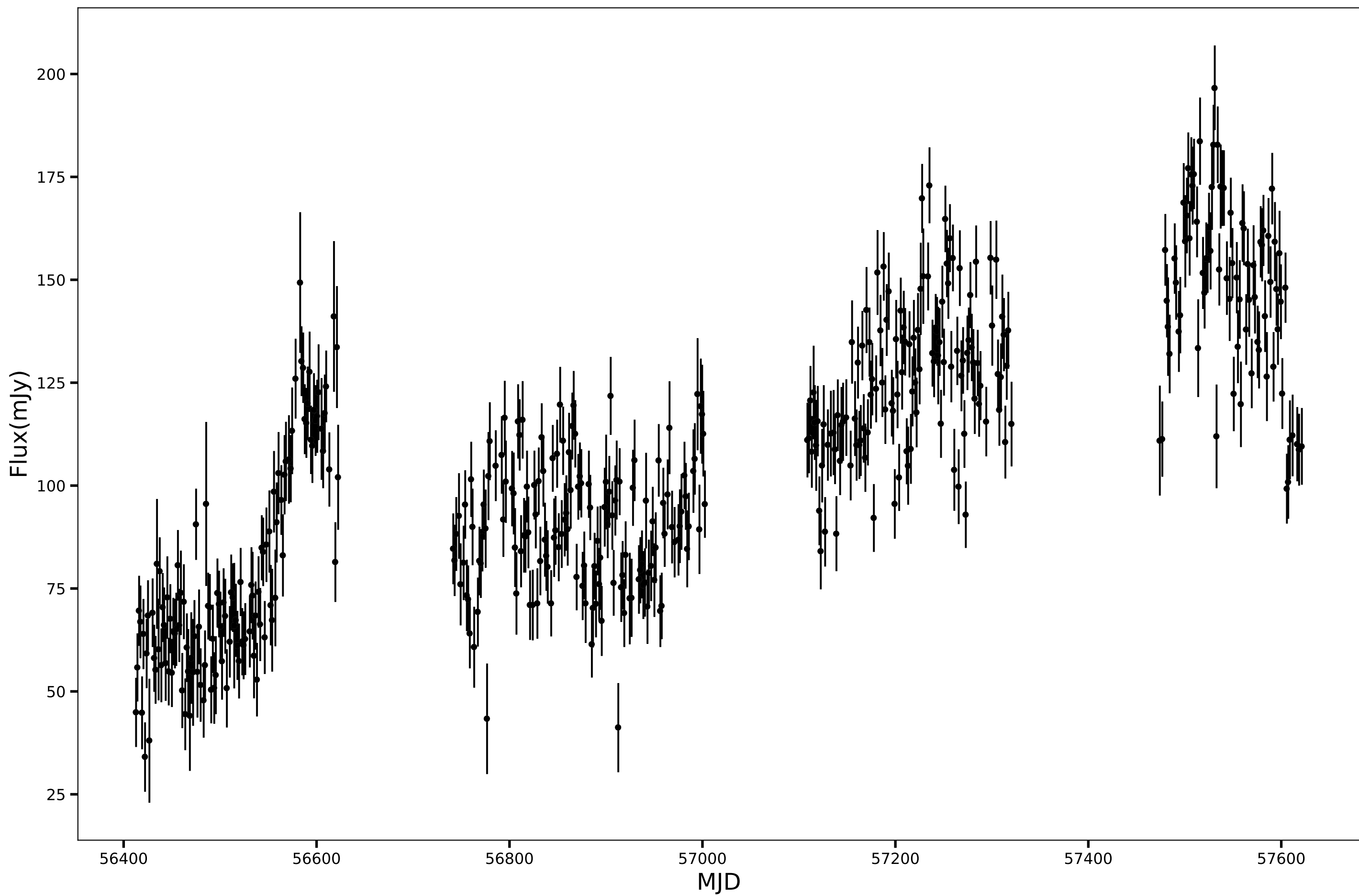
SPT-SJ015826-5810.9, RA=29.6114d, DEC=-58.1823d, mean_flux=106.06 (mJy), 150GHz
