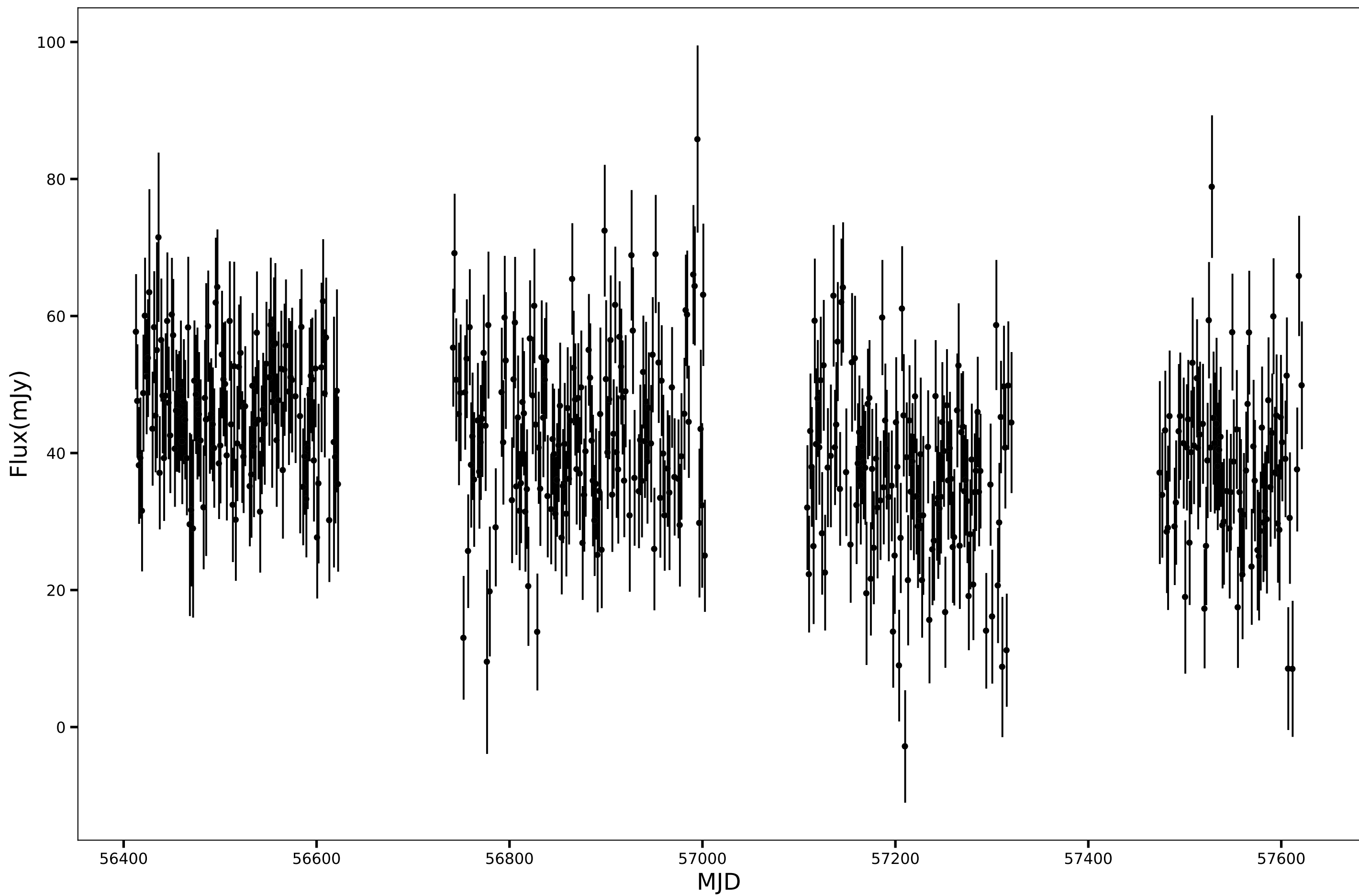
SPT-SJ015650-5439.7, RA=29.2110d, DEC=-54.6620d, mean_flux=41.51 (mJy), 150GHz
