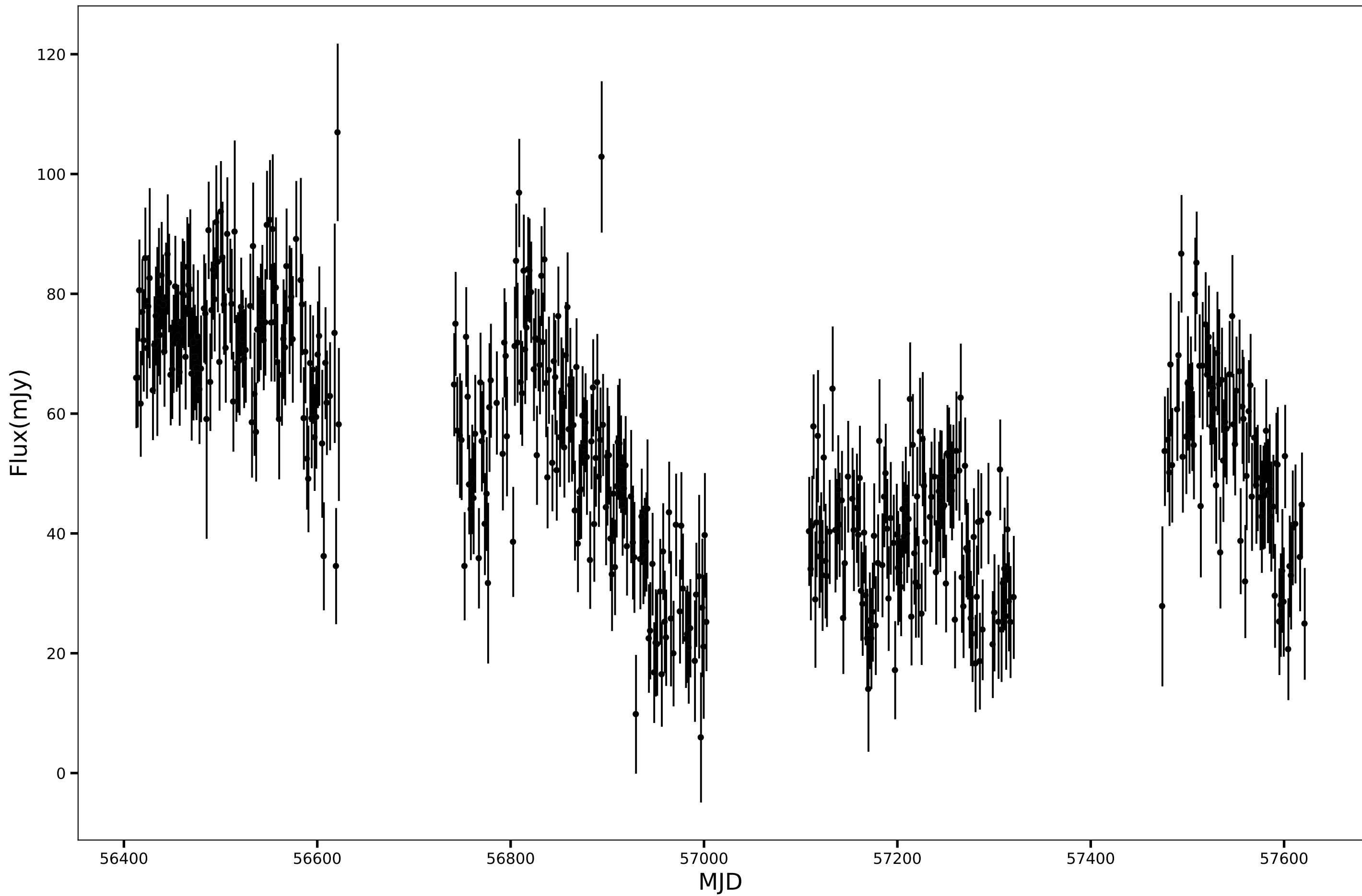
SPT-SJ015509-6425.5, RA=28.7913d, DEC=-64.4250d, mean_flux=53.76 (mJy), 150GHz
