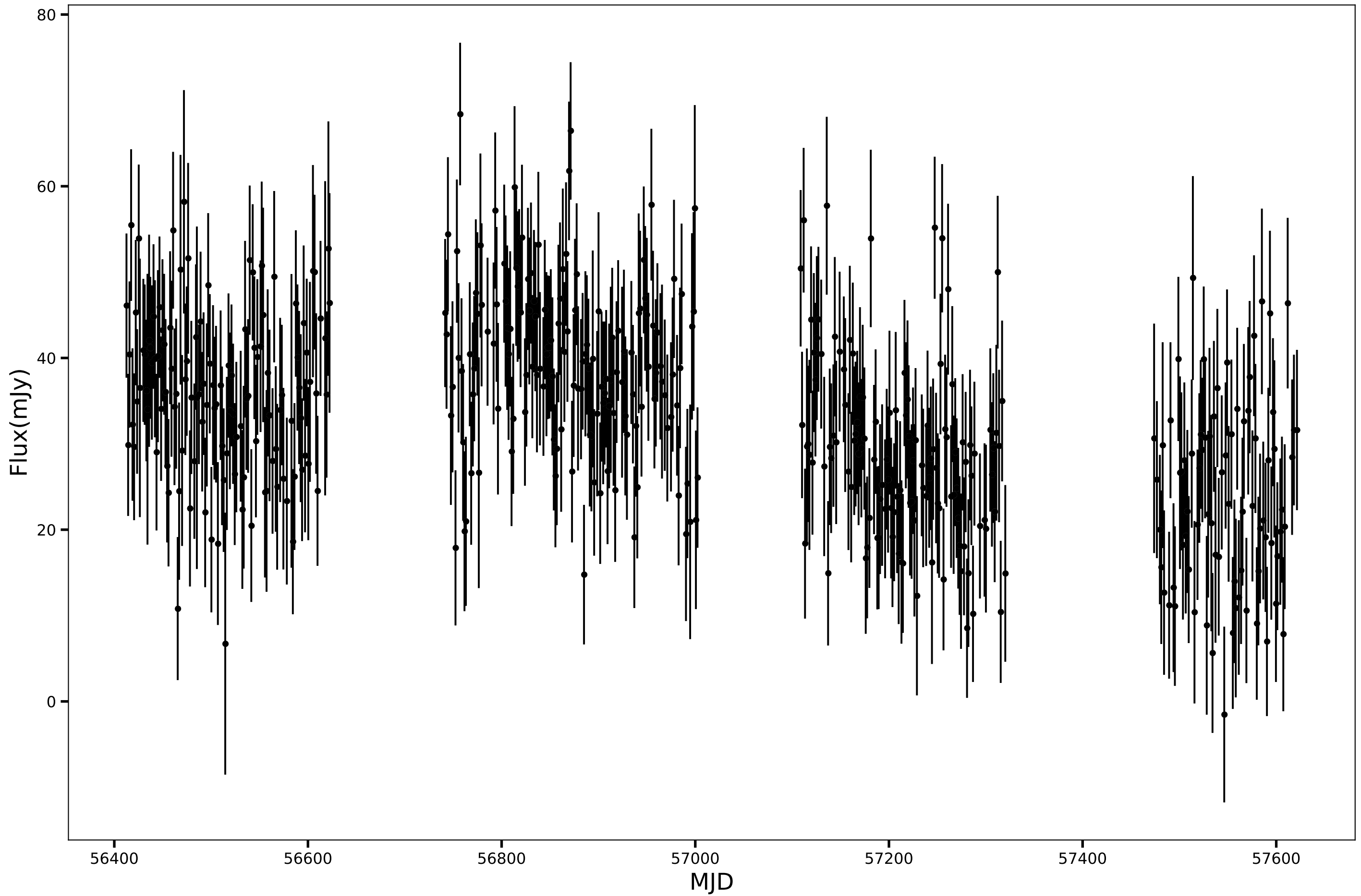
SPT-SJ015357-5406.8, RA=28.4912d, DEC=-54.1144d, mean_flux=33.13 (mJy), 150GHz
