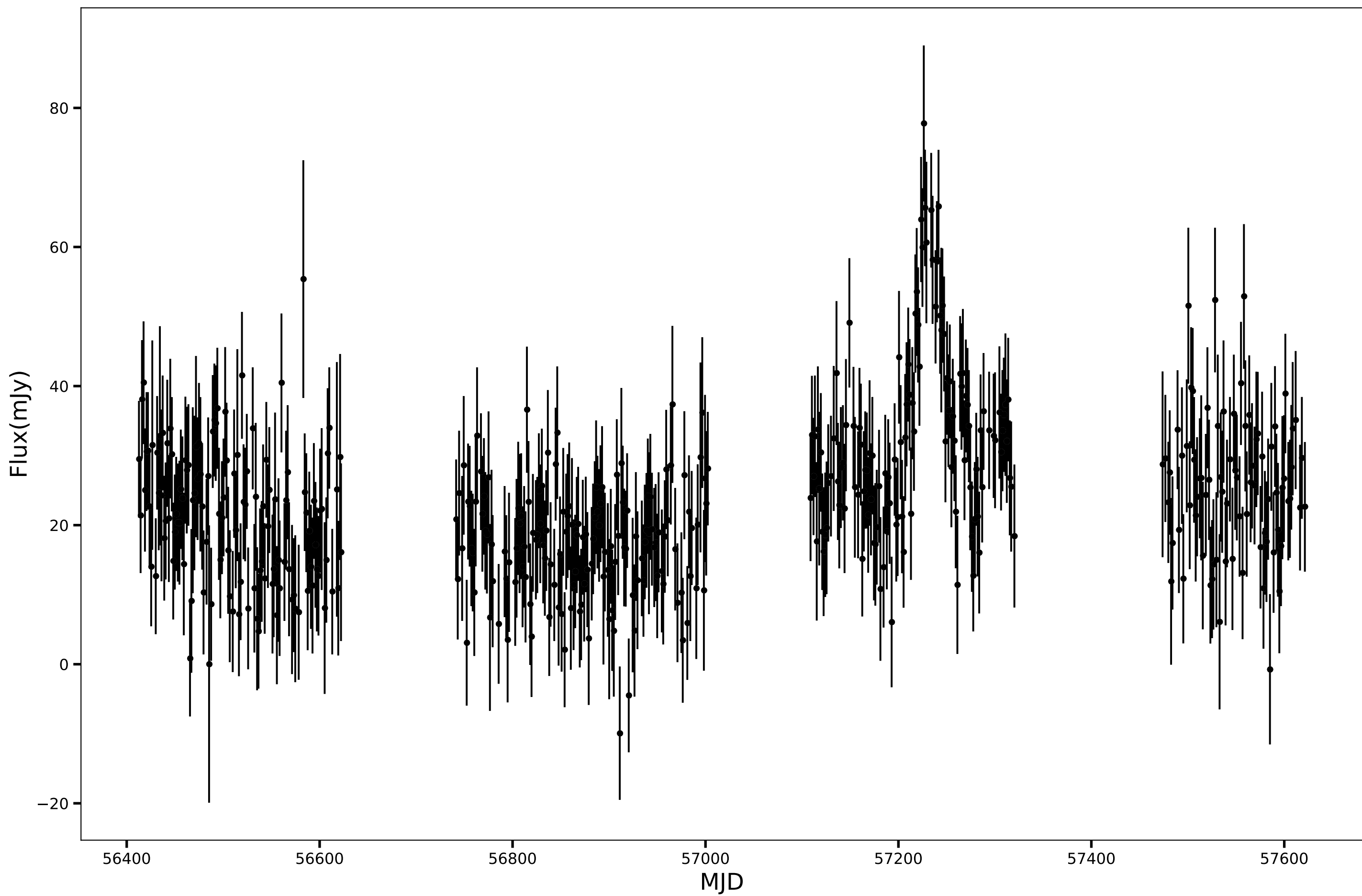
SPT-SJ015050-6044.2, RA=27.7096d, DEC=-60.7368d, mean_flux=23.76 (mJy), 150GHz
