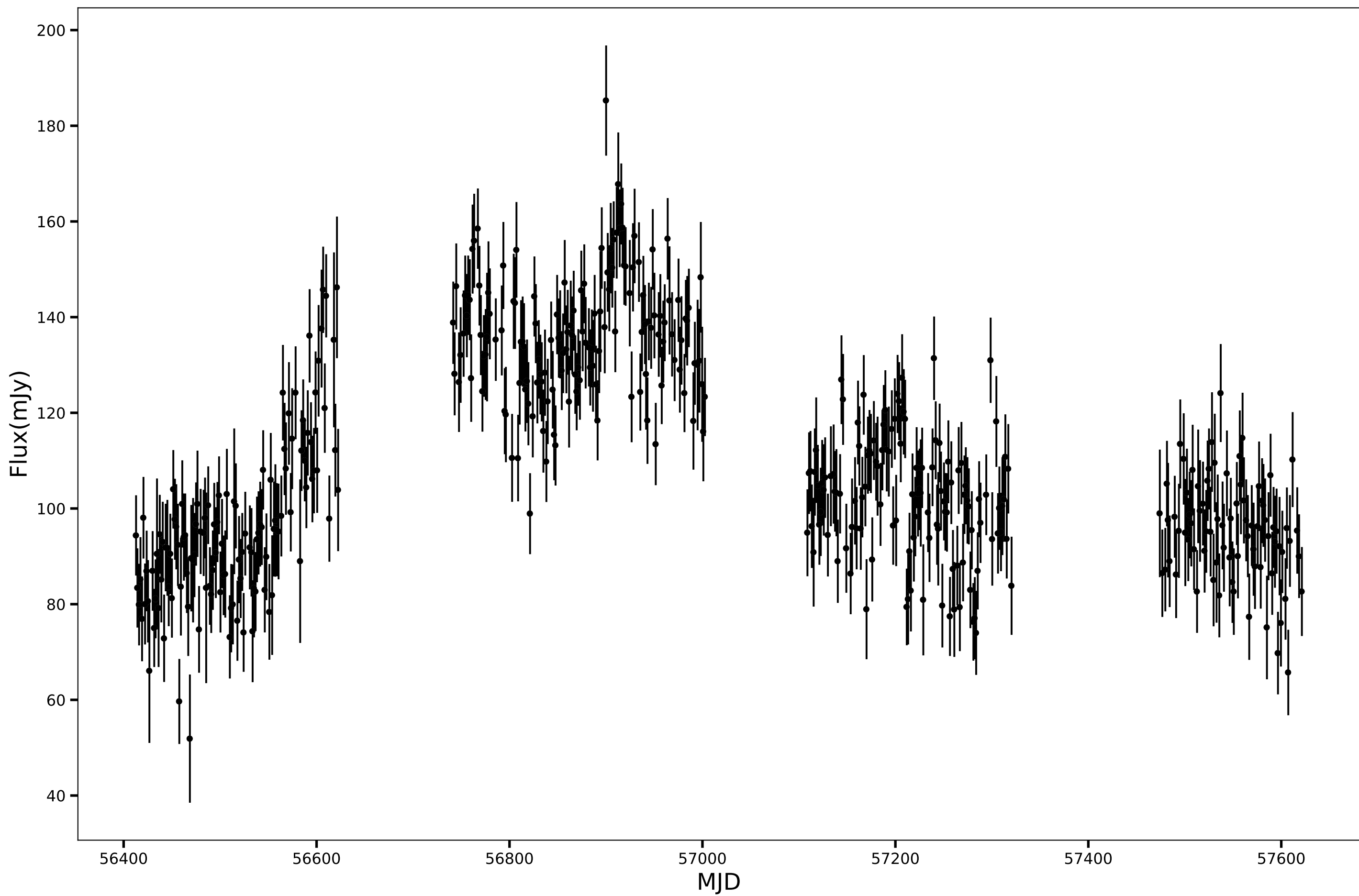
SPT-SJ014648-5202.5, RA=26.7001d, DEC=-52.0423d, mean_flux=109.72 (mJy), 150GHz
