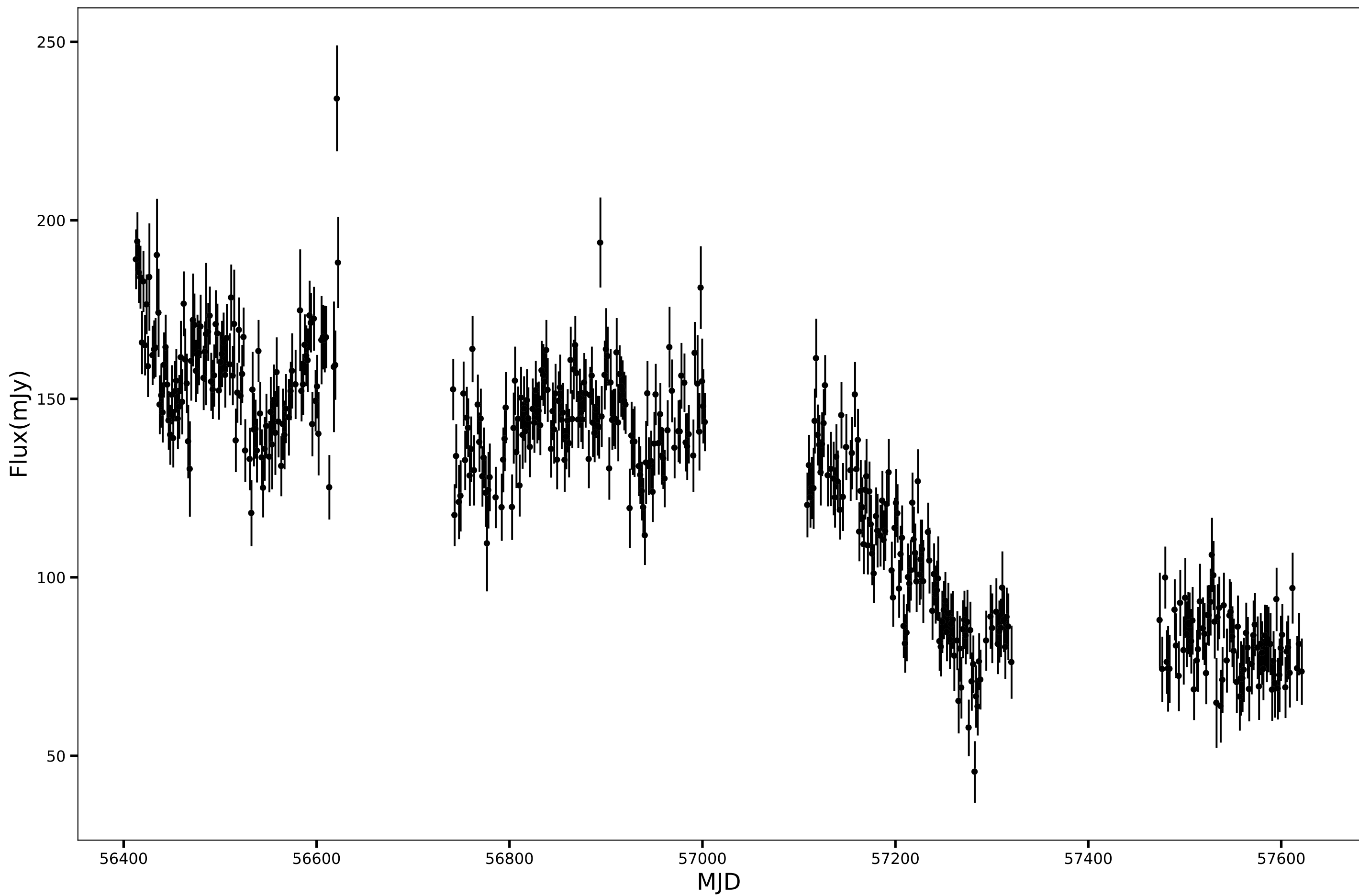
SPT-SJ014415-6421.8, RA=26.0657d, DEC=-64.3648d, mean_flux=126.29 (mJy), 150GHz
