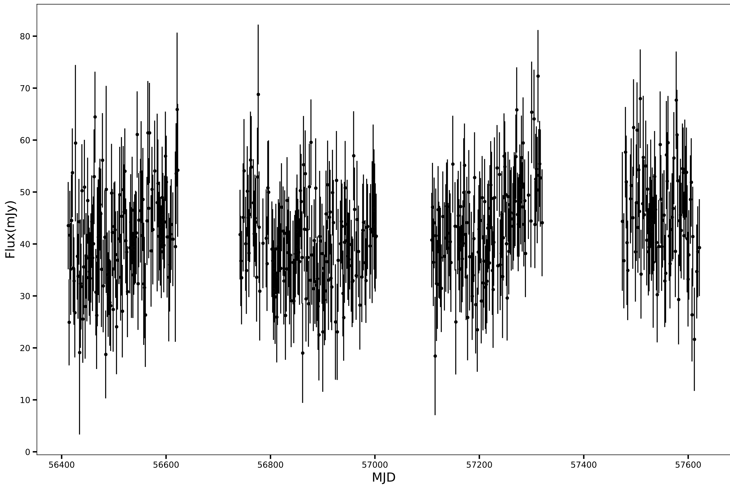
SPT-SJ014257-6044.9, RA=25.7376d, DEC=-60.7498d, mean_flux=42.06 (mJy), 150GHz
