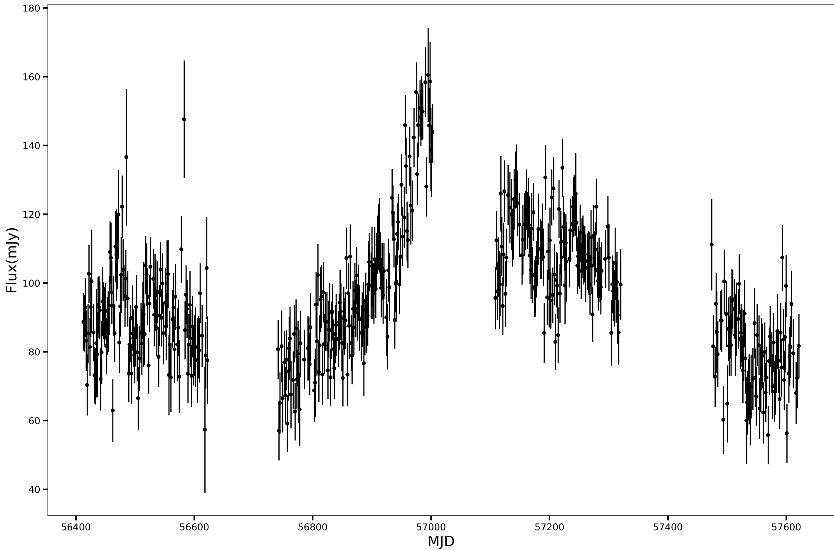
SPT-SJ014225-5729.8, RA=25.6081d, DEC=-57.4982d, mean_flux=95.52 (mJy), 150GHz
