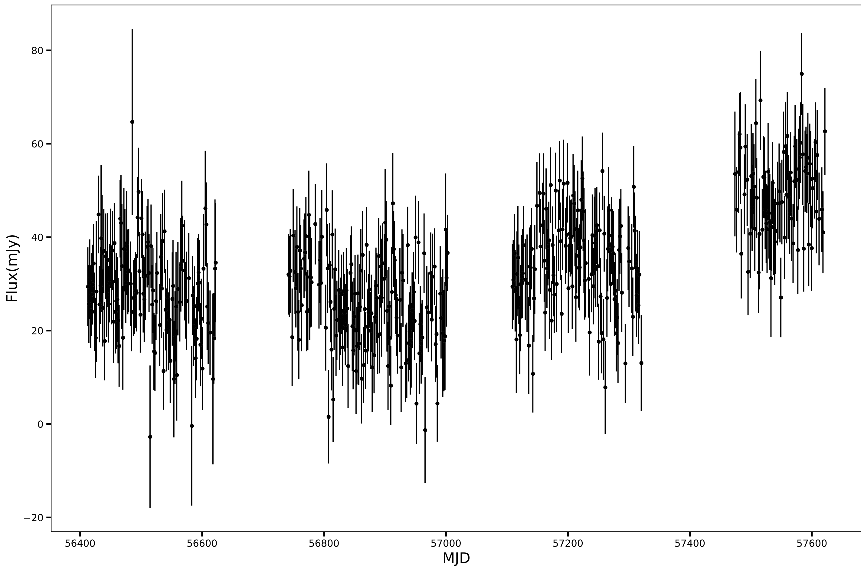
SPT-SJ014142-5650.6, RA=25.4274d, DEC=-56.8442d, mean_flux=32.74 (mJy), 150GHz
