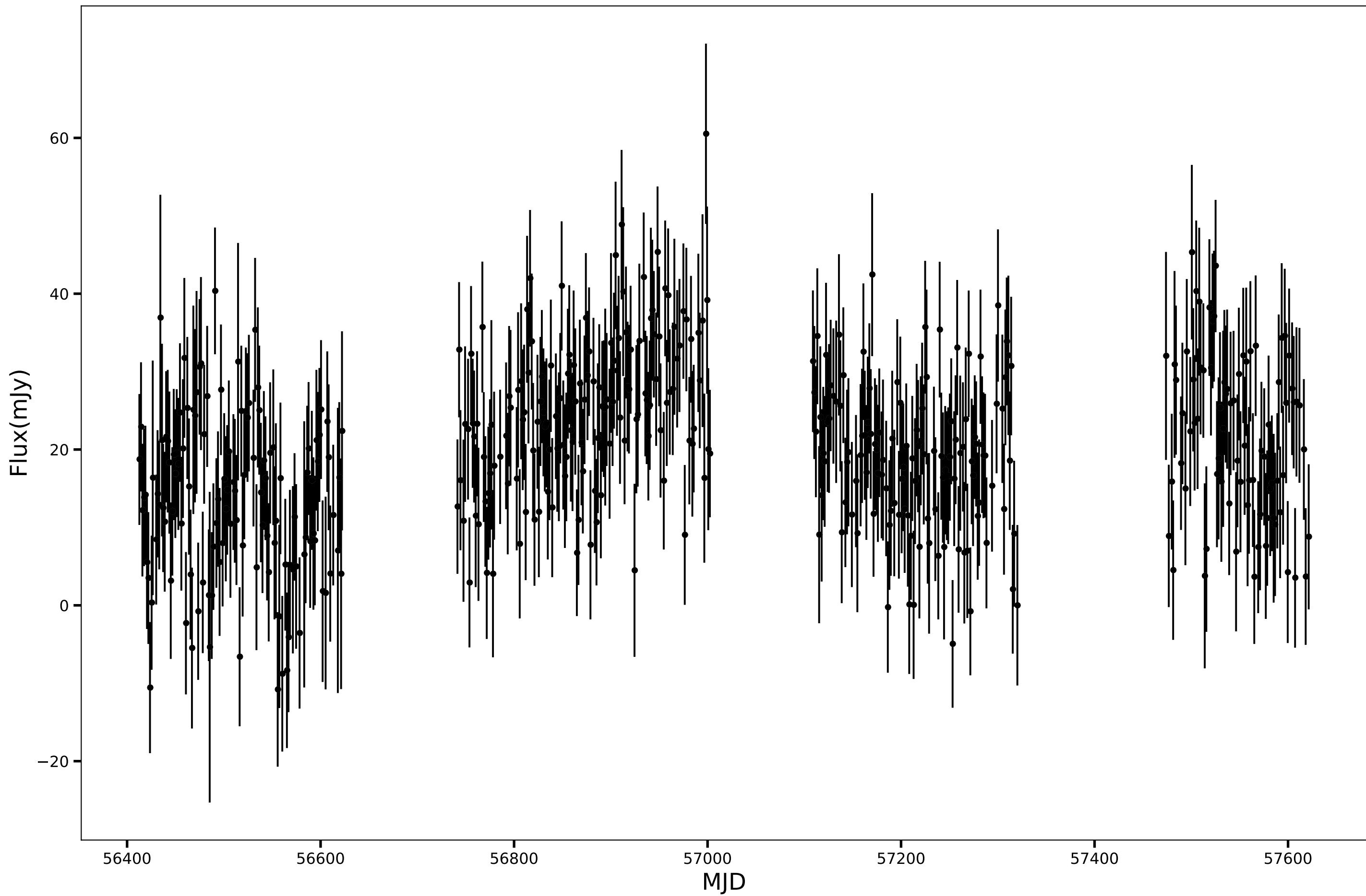
SPT-SJ013547-5244.2, RA=23.9472d, DEC=-52.7379d, mean_flux=19.91 (mJy), 150GHz
