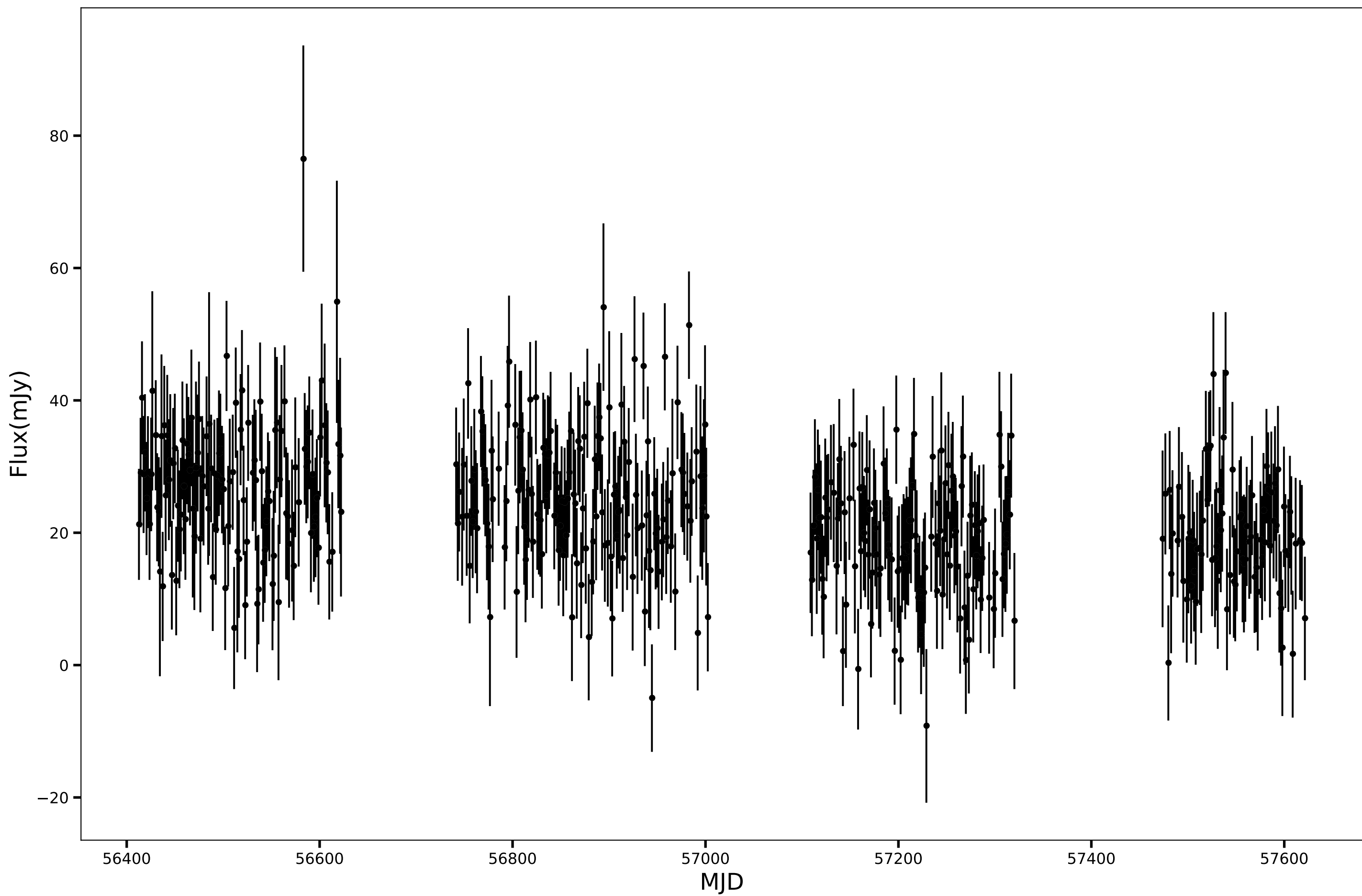
SPT-SJ013408-5526.3, RA=23.5375d, DEC=-55.4396d, mean_flux=23.13 (mJy), 150GHz
