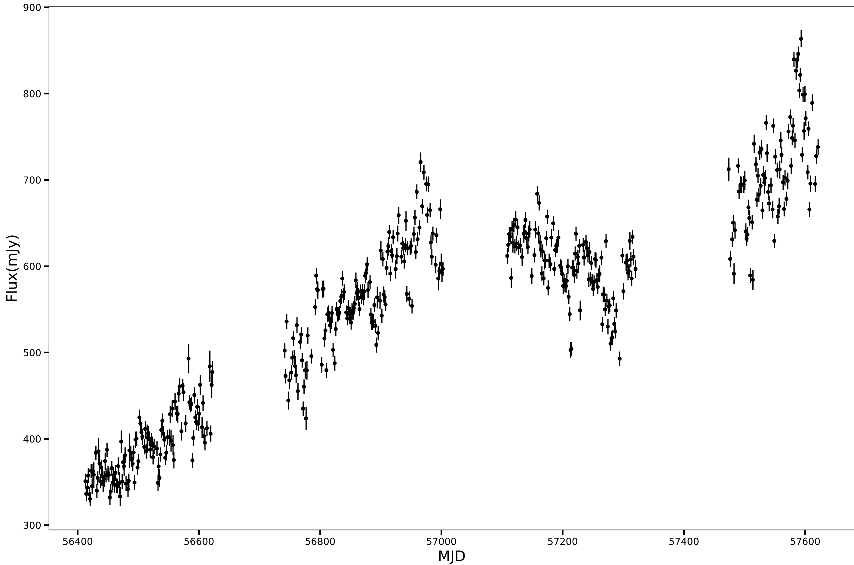
SPT-SJ013305-5200.1, RA=23.2711d, DEC=-52.0018d, mean_flux=554.15 (mJy), 150GHz
