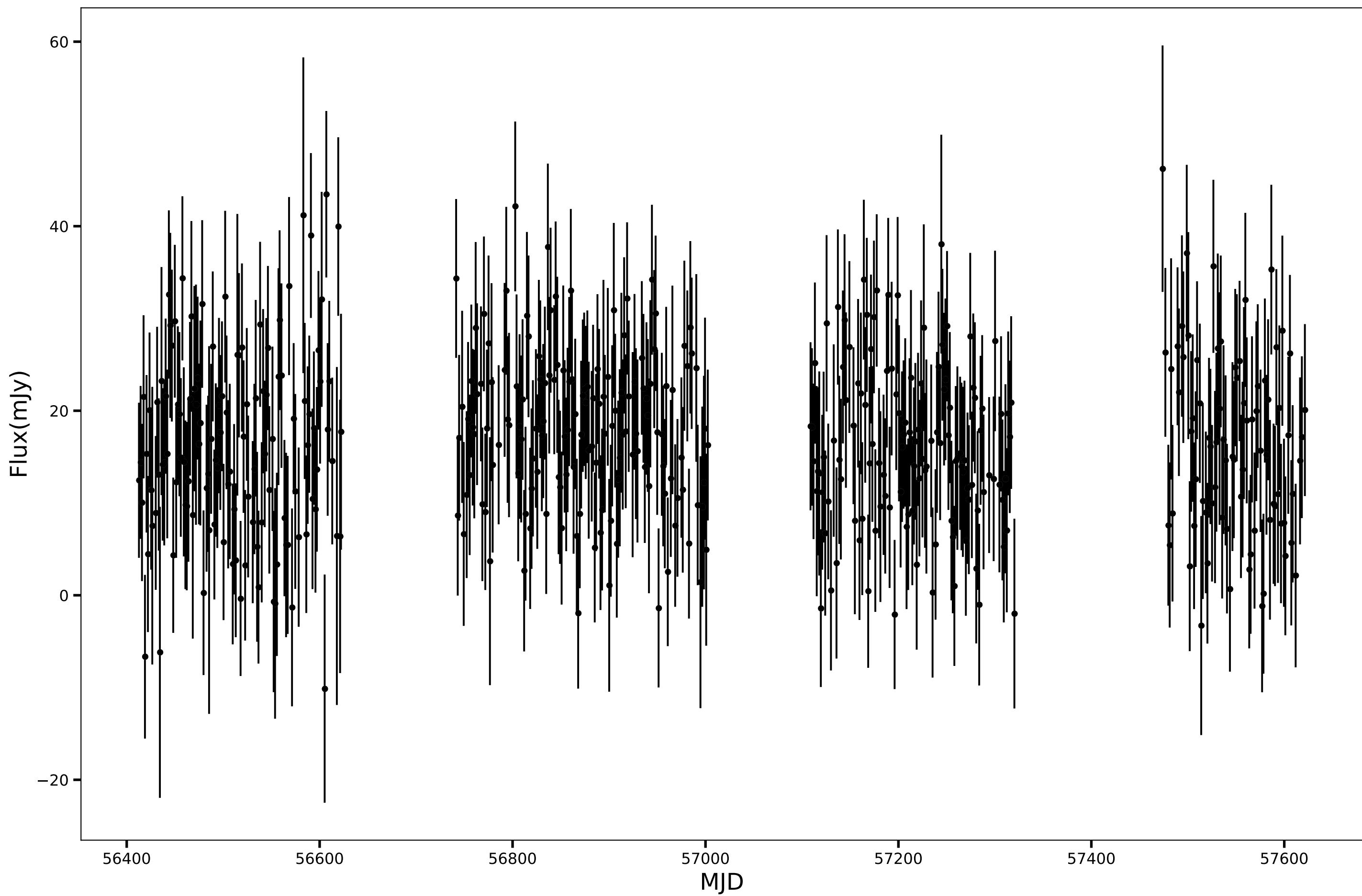
SPT-SJ012833-5255.3, RA=22.1397d, DEC=-52.9219d, mean_flux=16.69 (mJy), 150GHz
