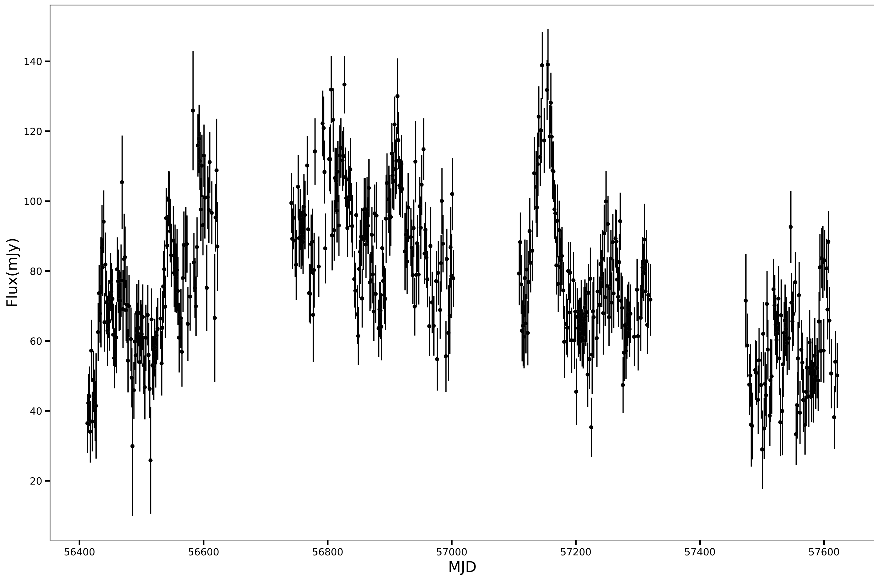
SPT-SJ012820-5649.6, RA=22.0855d, DEC=-56.8276d, mean_flux=77.24 (mJy), 150GHz
