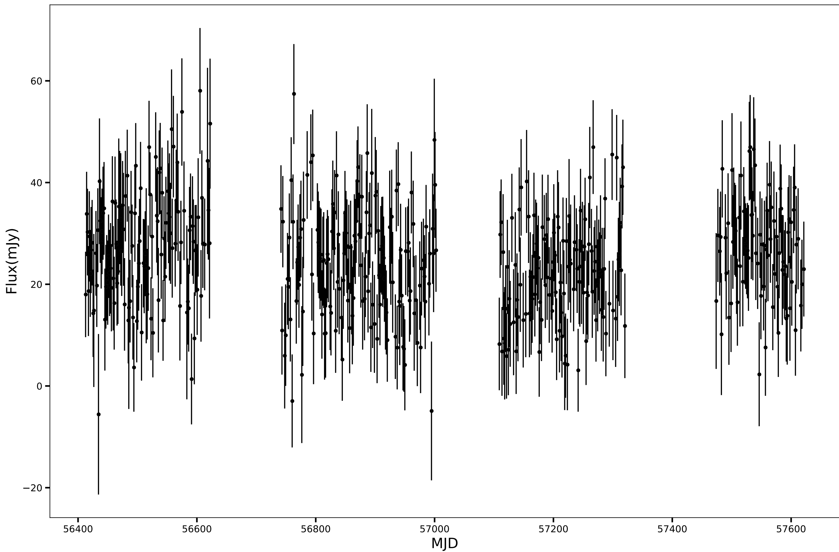
SPT-SJ012623-5103.1, RA=21.5982d, DEC=-51.0520d, mean_flux=24.83 (mJy), 150GHz
