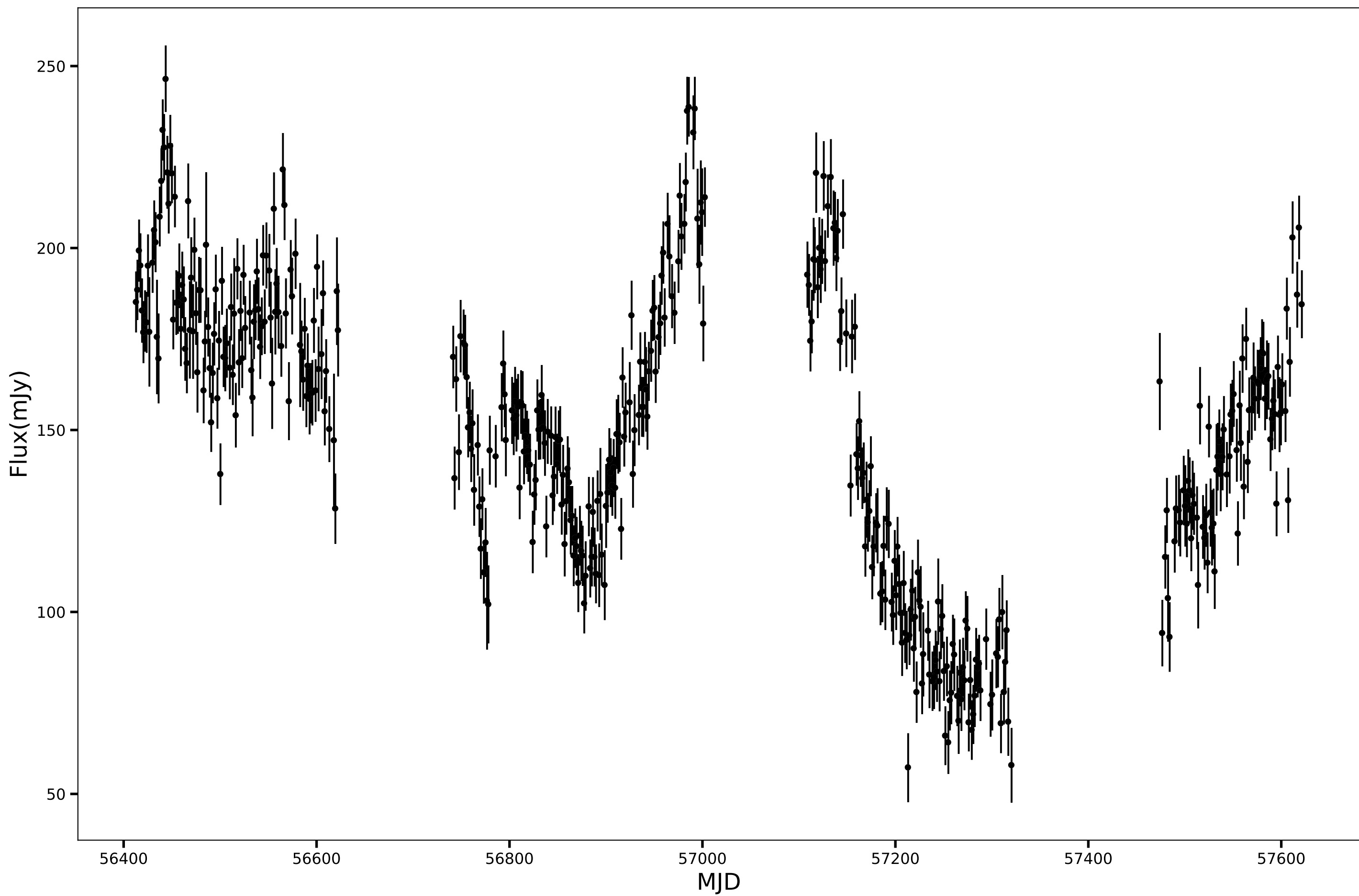
SPT-SJ012456-5113.1, RA=21.2366d, DEC=-51.2199d, mean_flux=149.94 (mJy), 150GHz
