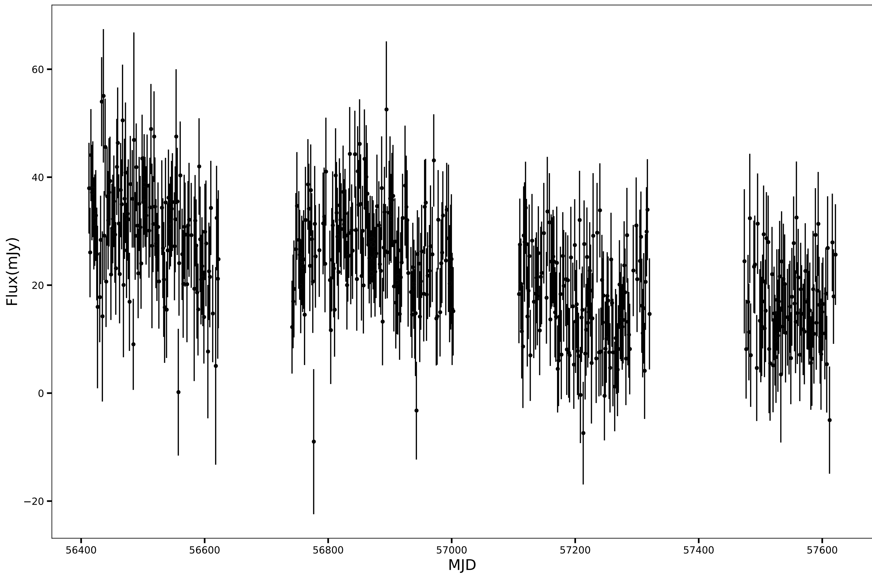
SPT-SJ012140-6309.2, RA=20.4188d, DEC=-63.1536d, mean_flux=23.25 (mJy), 150GHz
