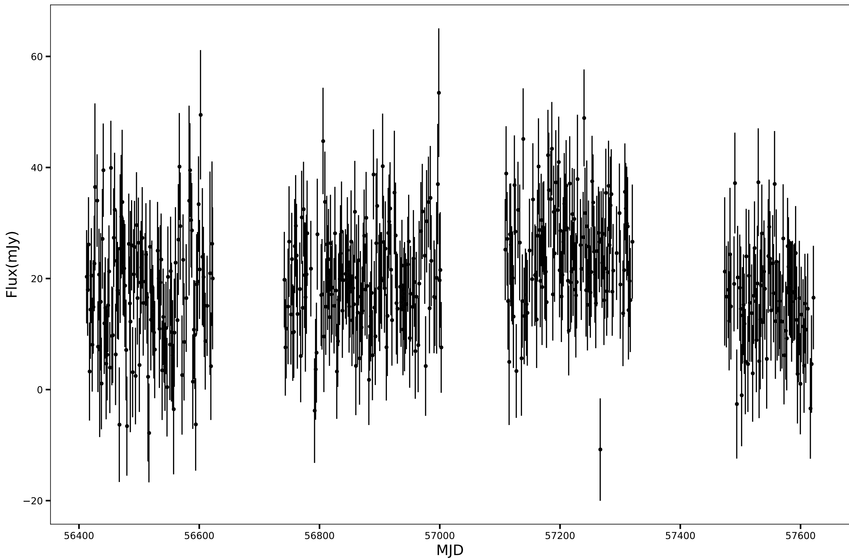
SPT-SJ012007-5211.1, RA=20.0314d, DEC=-52.1858d, mean_flux=19.62 (mJy), 150GHz
