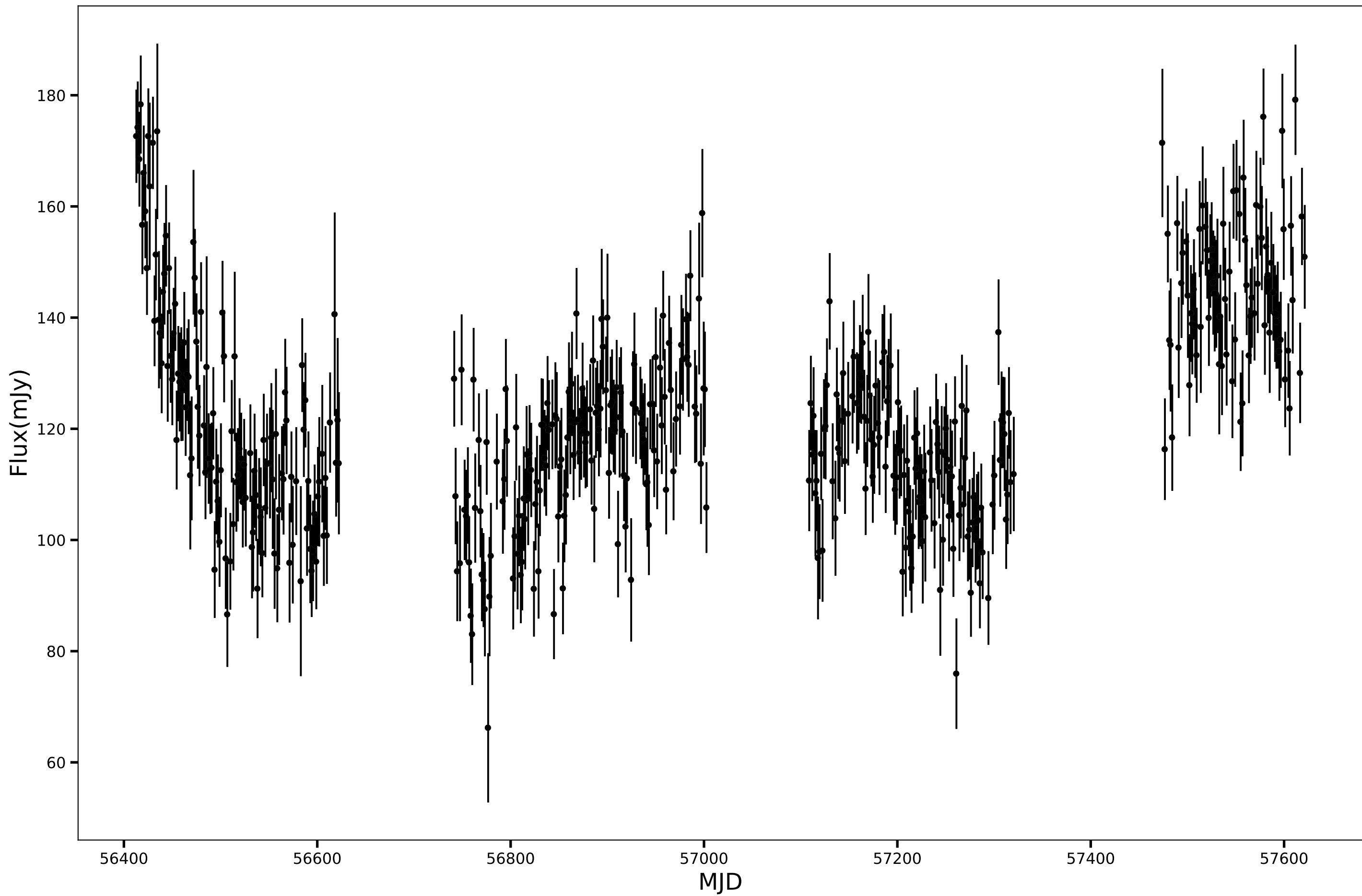
SPT-SJ011950-5357.2, RA=19.9614d, DEC=-53.9546d, mean_flux=122.00 (mJy), 150GHz
