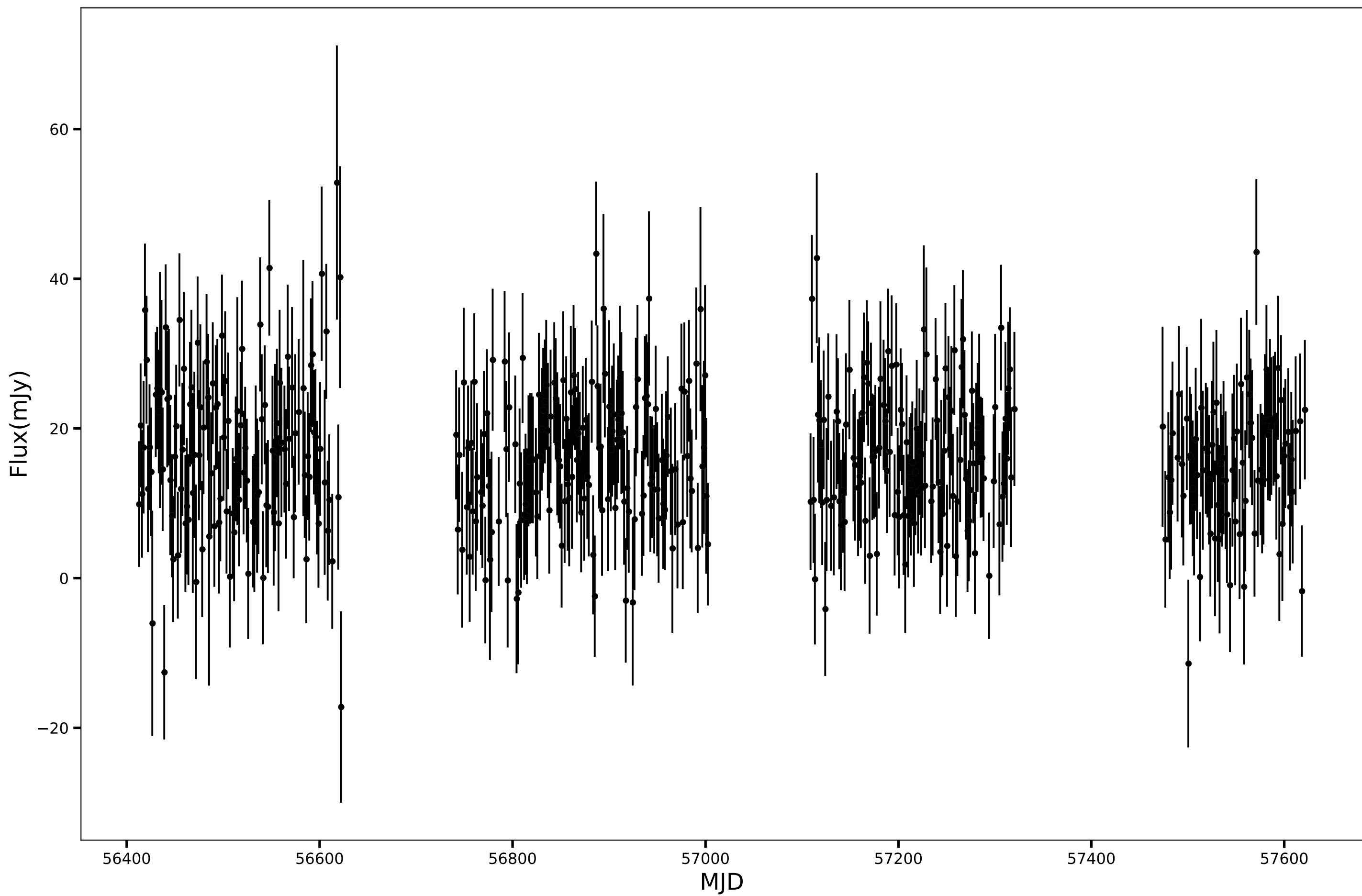
SPT-SJ011323-5329.8, RA=18.3475d, DEC=-53.4973d, mean_flux=16.19 (mJy), 150GHz
