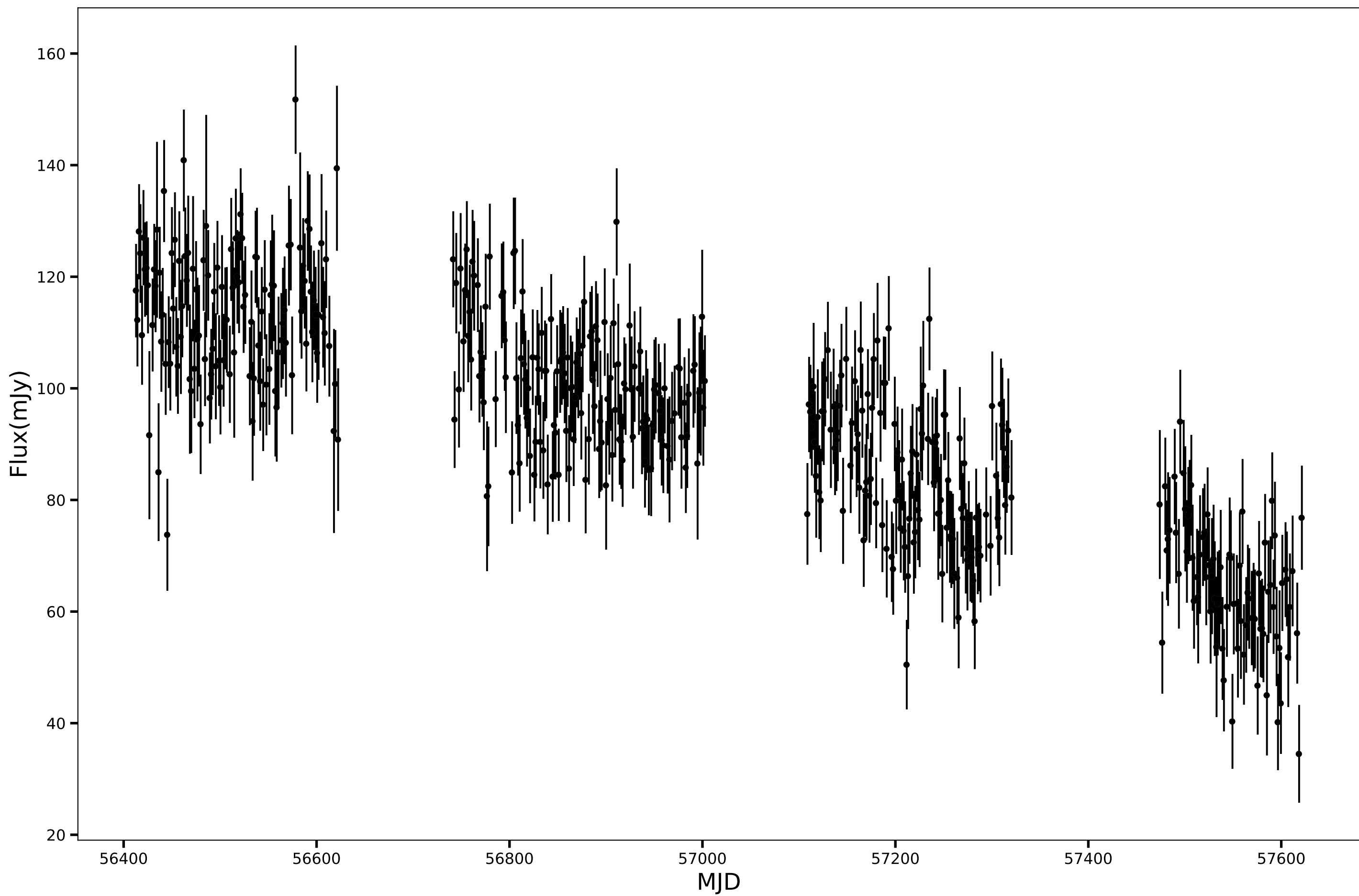
SPT-SJ011016-6316.0, RA=17.5688d, DEC=-63.2669d, mean_flux=93.65 (mJy), 150GHz
