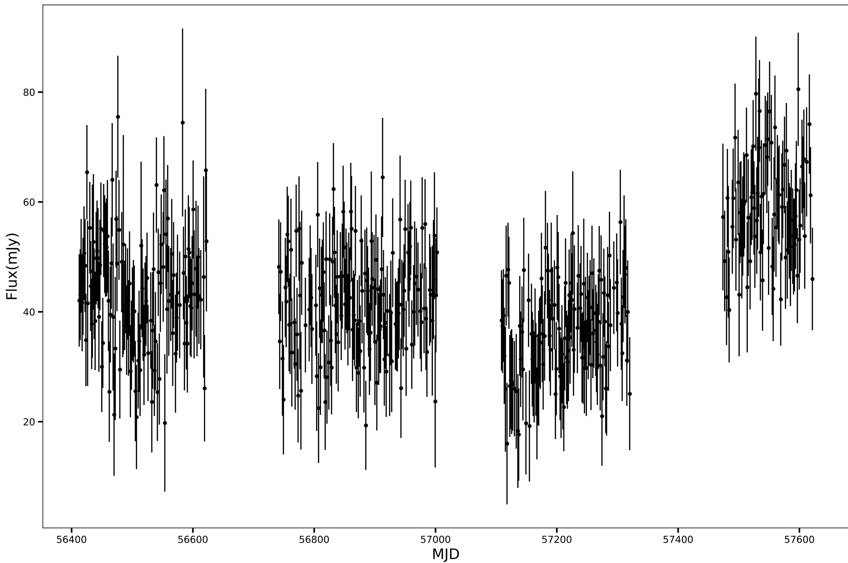
SPT-SJ010406-5657.3, RA=16.0288d, DEC=-56.9554d, mean_flux=43.58 (mJy), 150GHz
