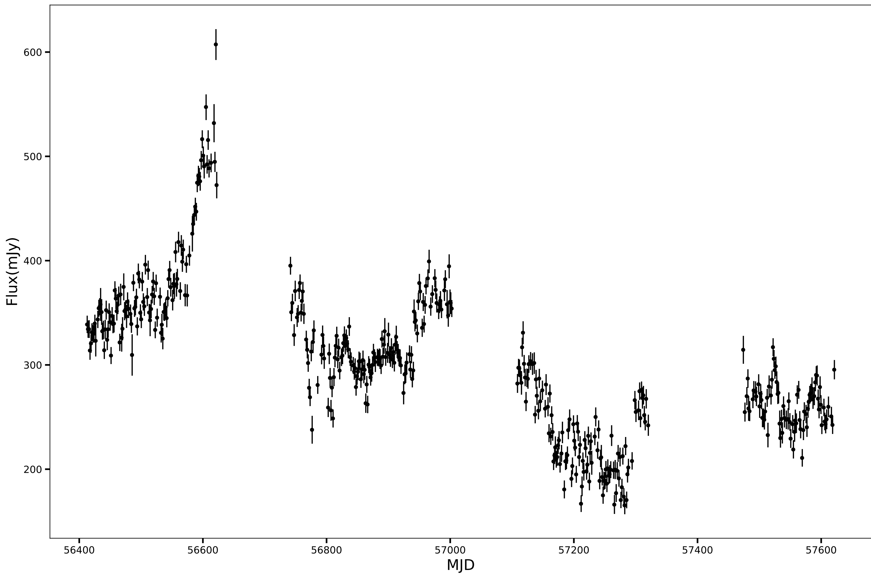
SPT-SJ010333-6439.2, RA=15.8895d, DEC=-64.6536d, mean_flux=303.18 (mJy), 150GHz
