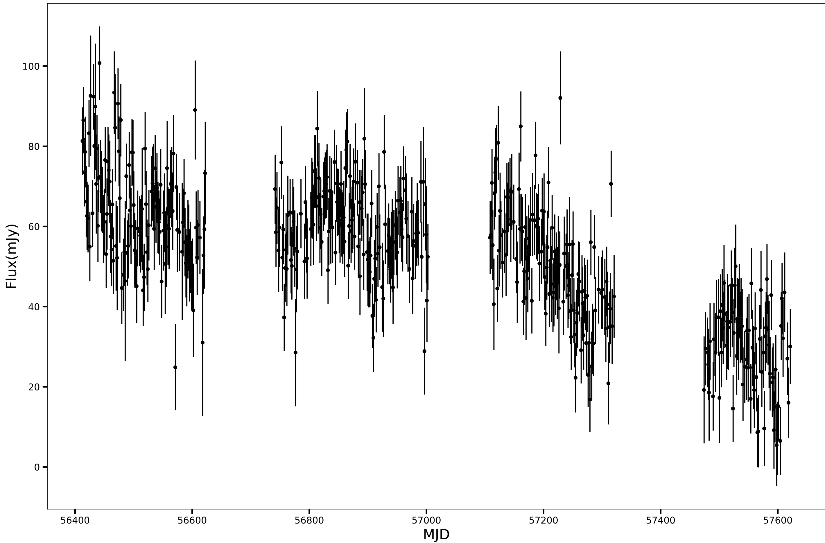
SPT-SJ010306-5109.1, RA=15.7758d, DEC=-51.1525d, mean_flux=53.15 (mJy), 150GHz
