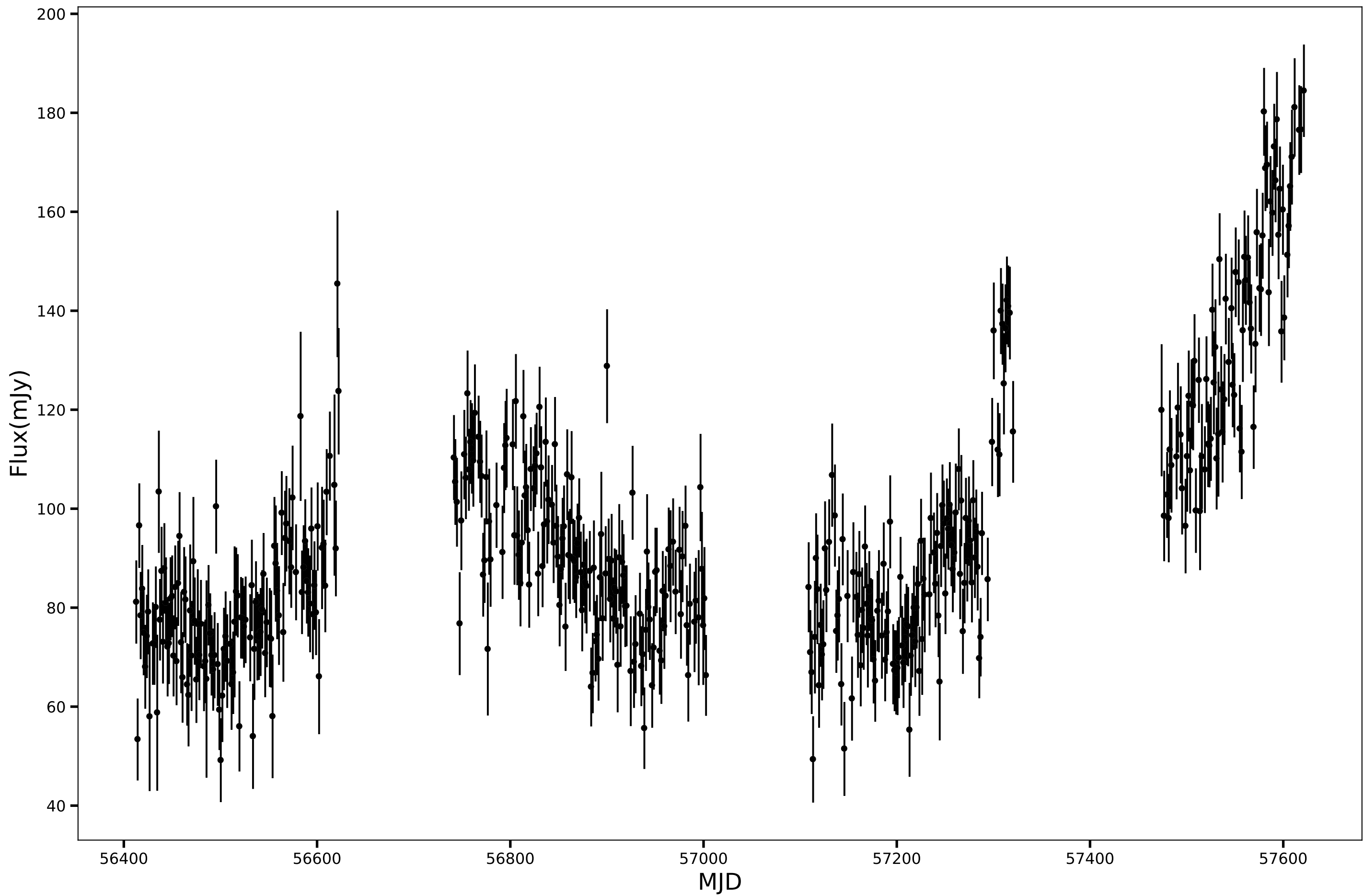
SPT-SJ010210-5637.2, RA=15.5421d, DEC=-56.6204d, mean_flux=94.45 (mJy), 150GHz
