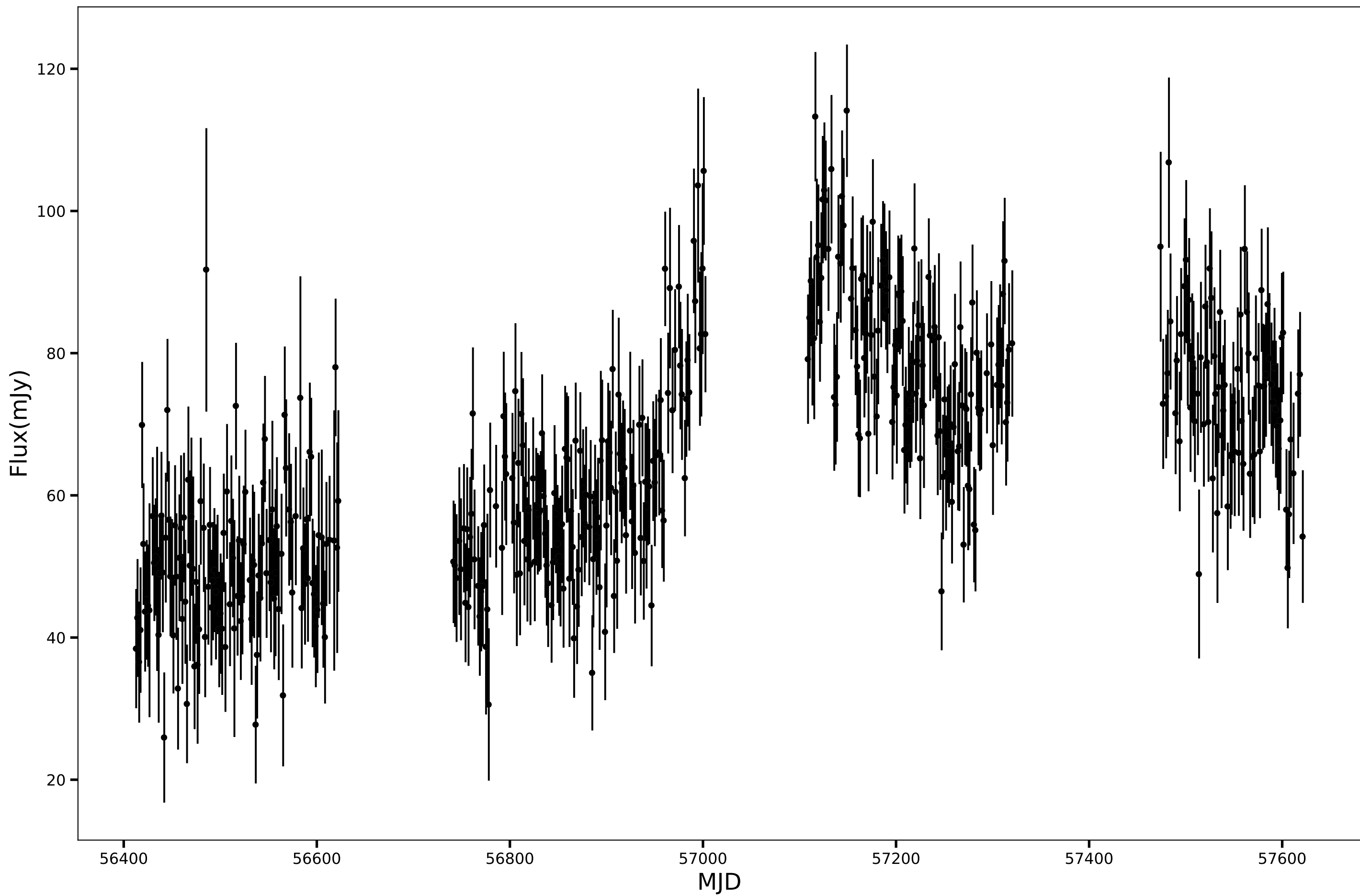
SPT-SJ010115-6233.2, RA=15.3127d, DEC=-62.5533d, mean_flux=65.31 (mJy), 150GHz
