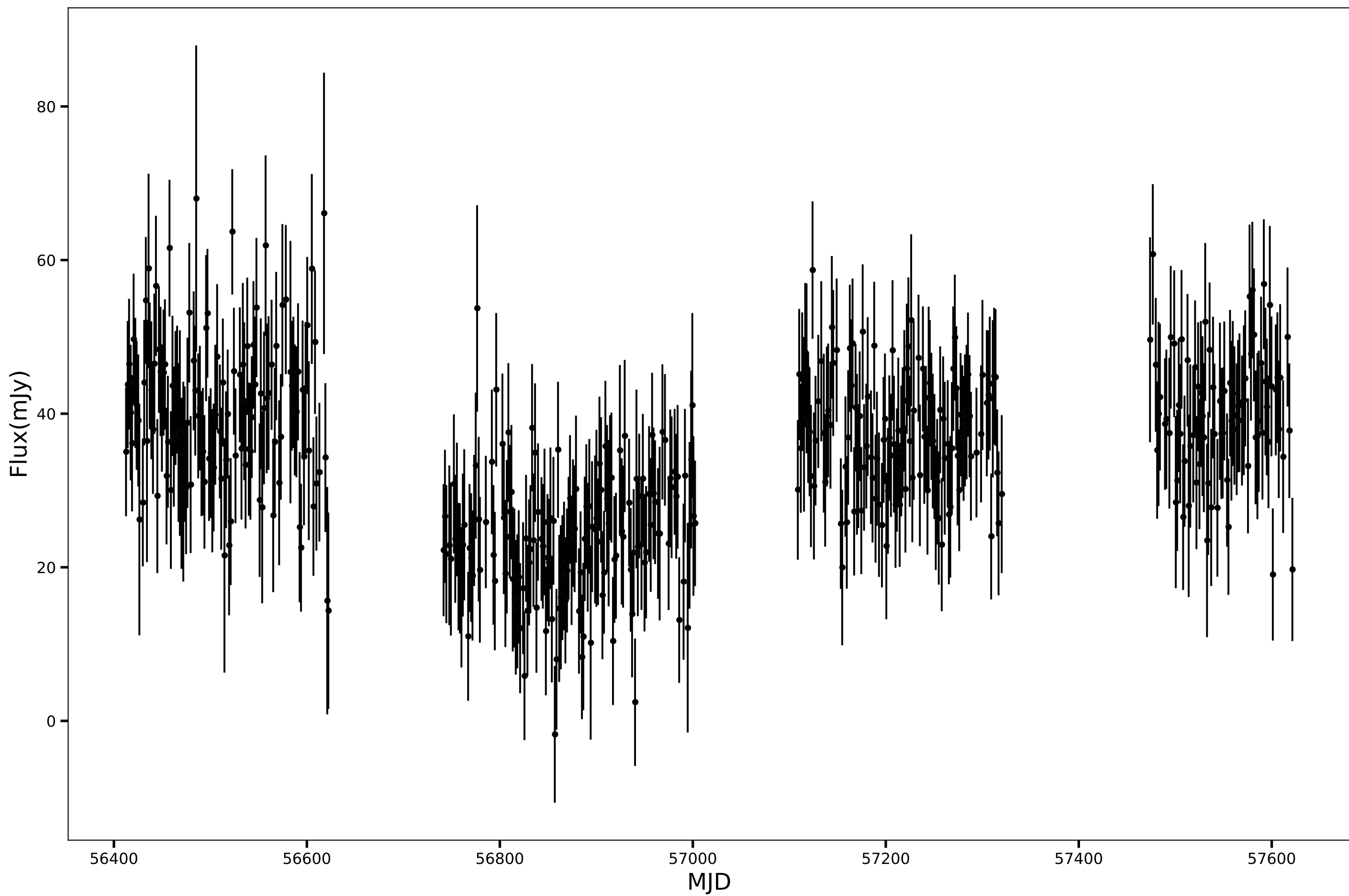
SPT-SJ005920-6126.8, RA=14.8358d, DEC=-61.4479d, mean_flux=34.49 (mJy), 150GHz
