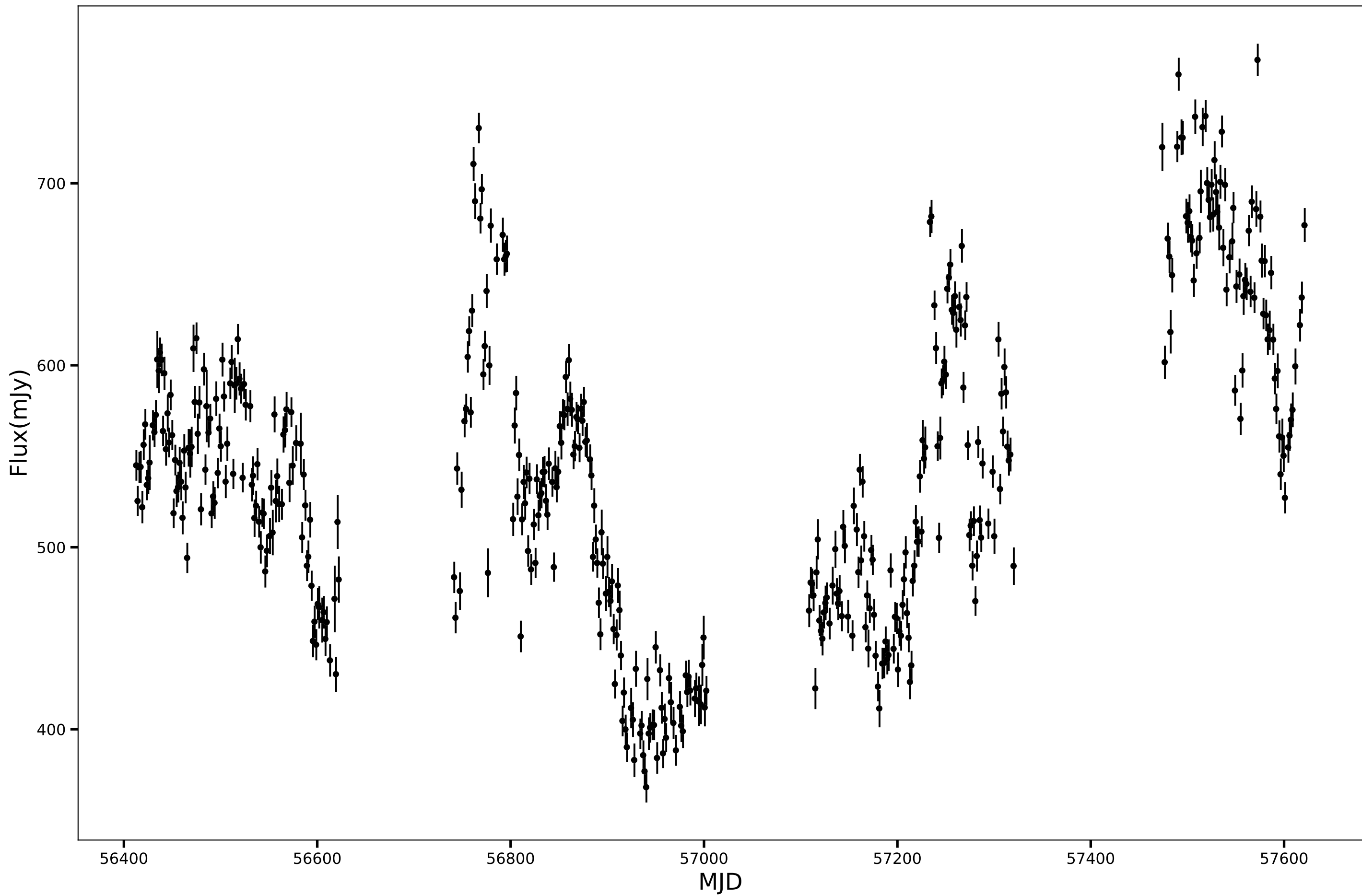
SPT-SJ005846-5659.1, RA=14.6944d, DEC=-56.9855d, mean_flux=542.82 (mJy), 150GHz
