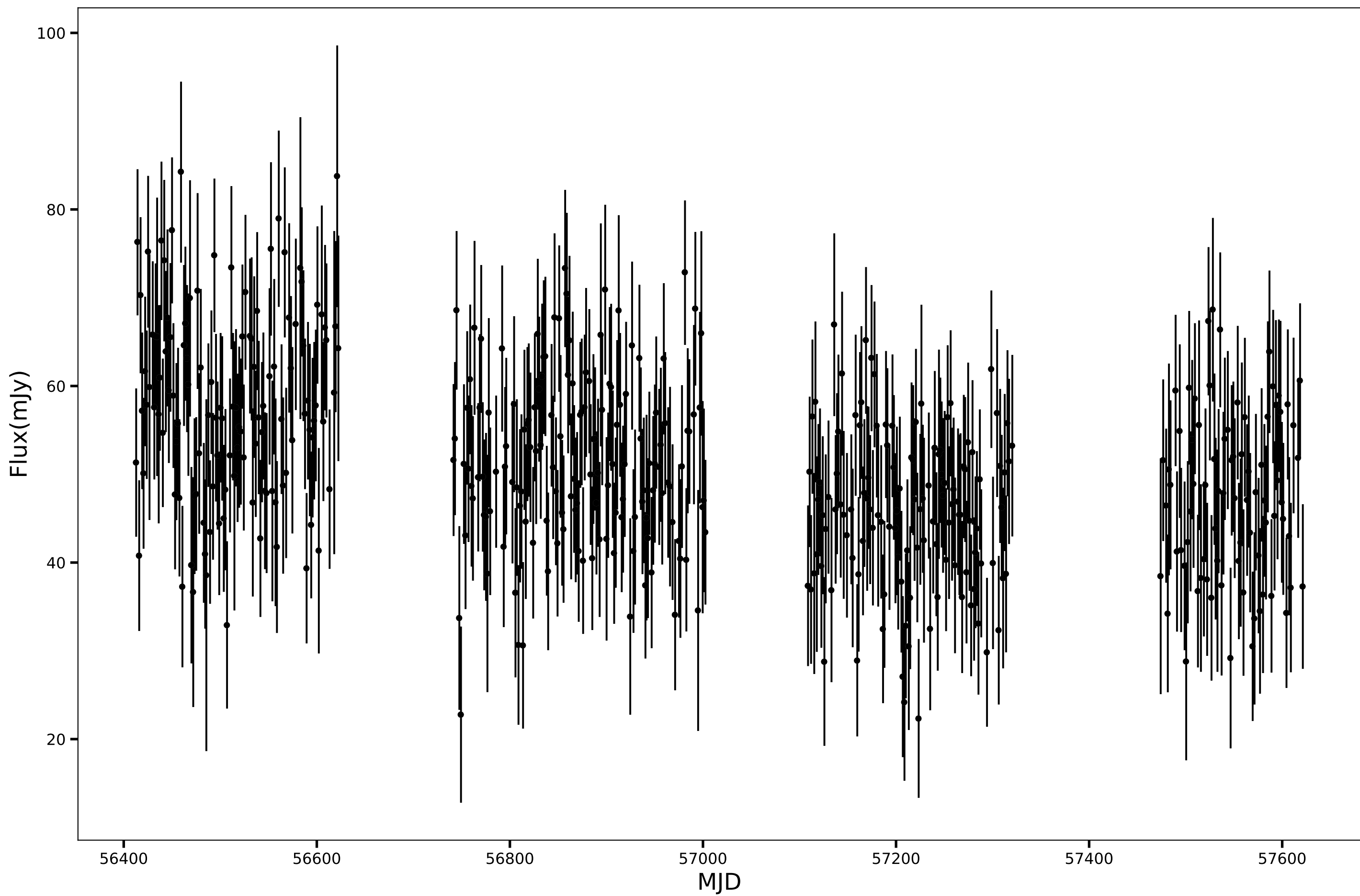
SPT-SJ005705-5214.3, RA=14.2738d, DEC=-52.2392d, mean_flux=51.08 (mJy), 150GHz
