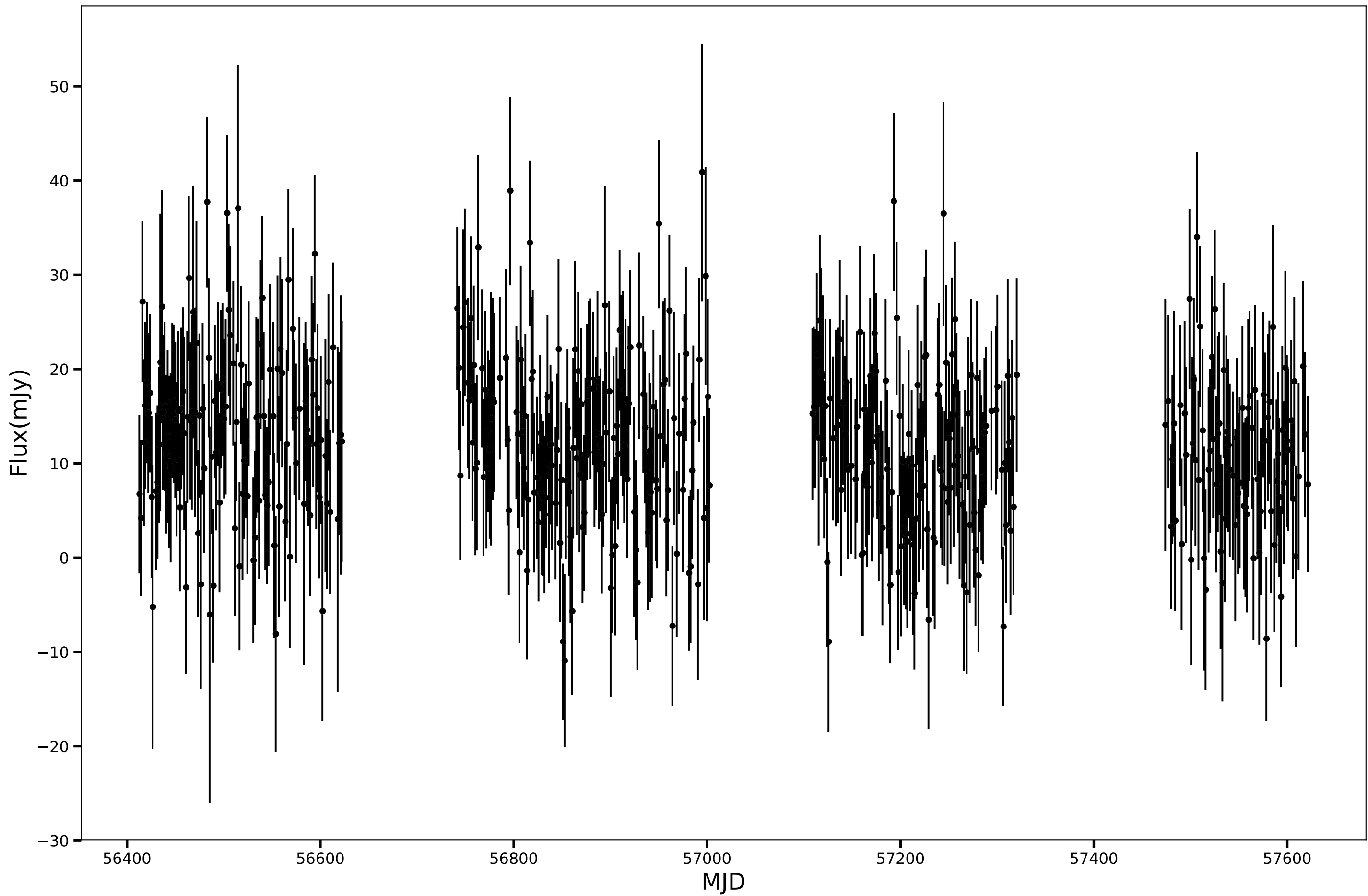
SPT-SJ003813-6112.8, RA=9.5554d, DEC=-61.2139d, mean_flux=11.98 (mJy), 150GHz
